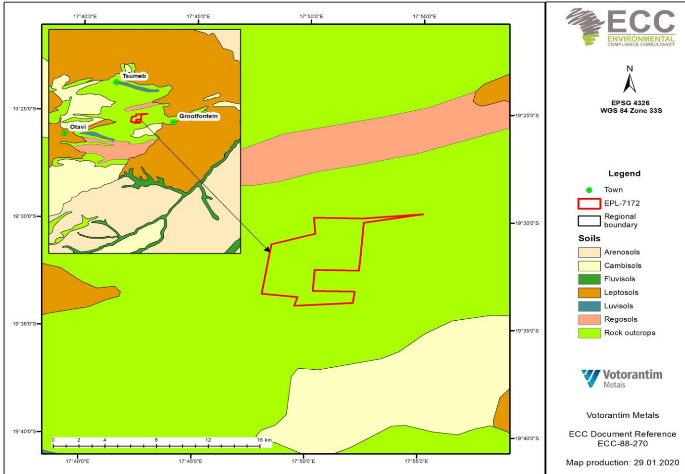
FIGURE 7 - EPL 7172 REGIONAL AND LOCAL SOIL MAP
