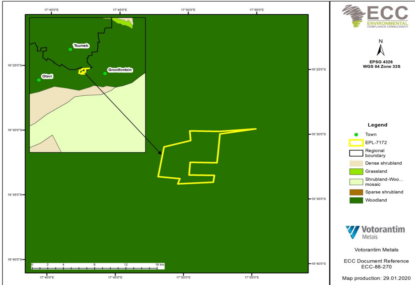
FIGURE 10 - EPL 7172 REGIONAL AND LOCAL VEGETATION MAP
