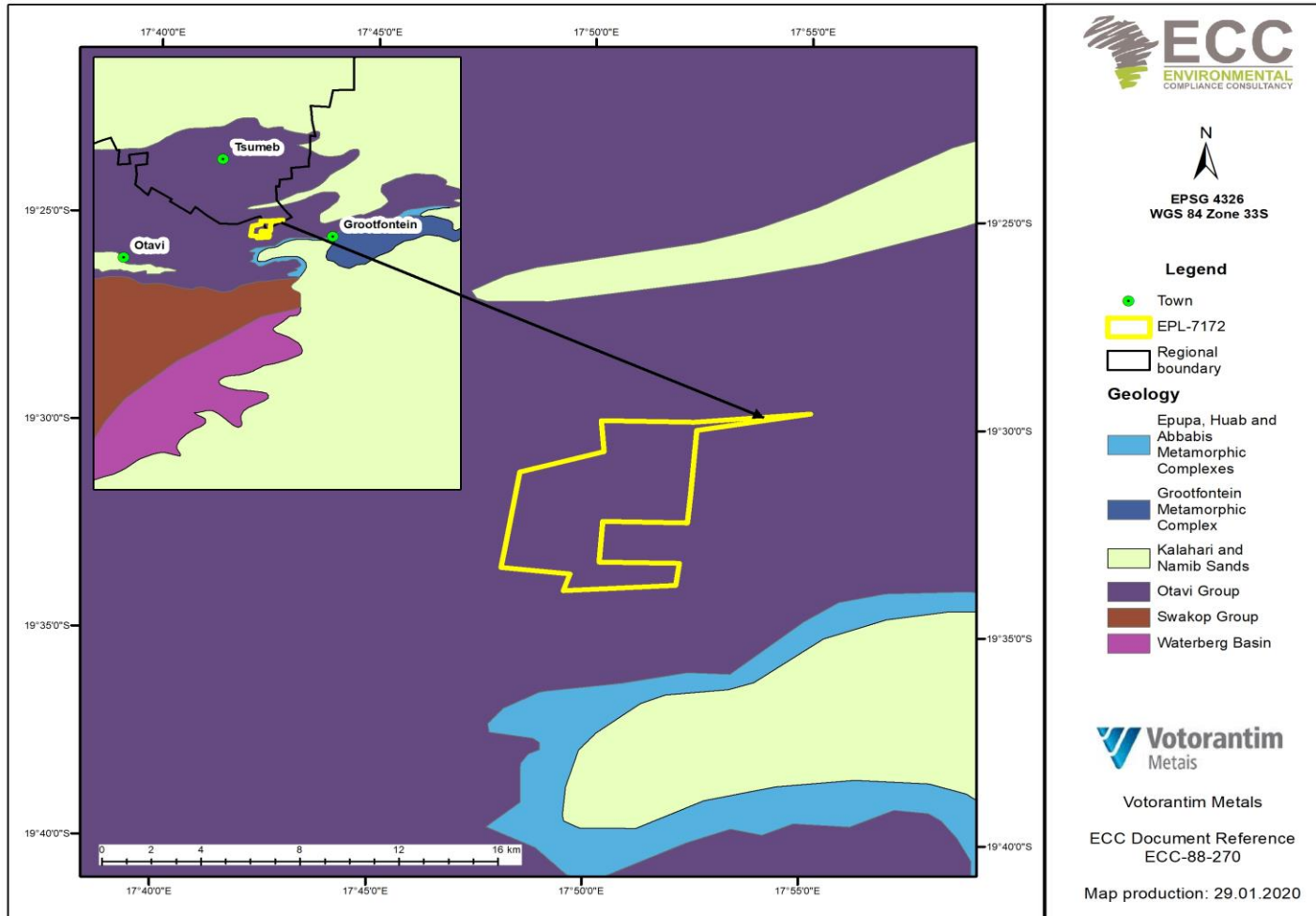
FIGURE 6 - EPL 7172 REGIONAL AND LOCAL GEOLOGY
