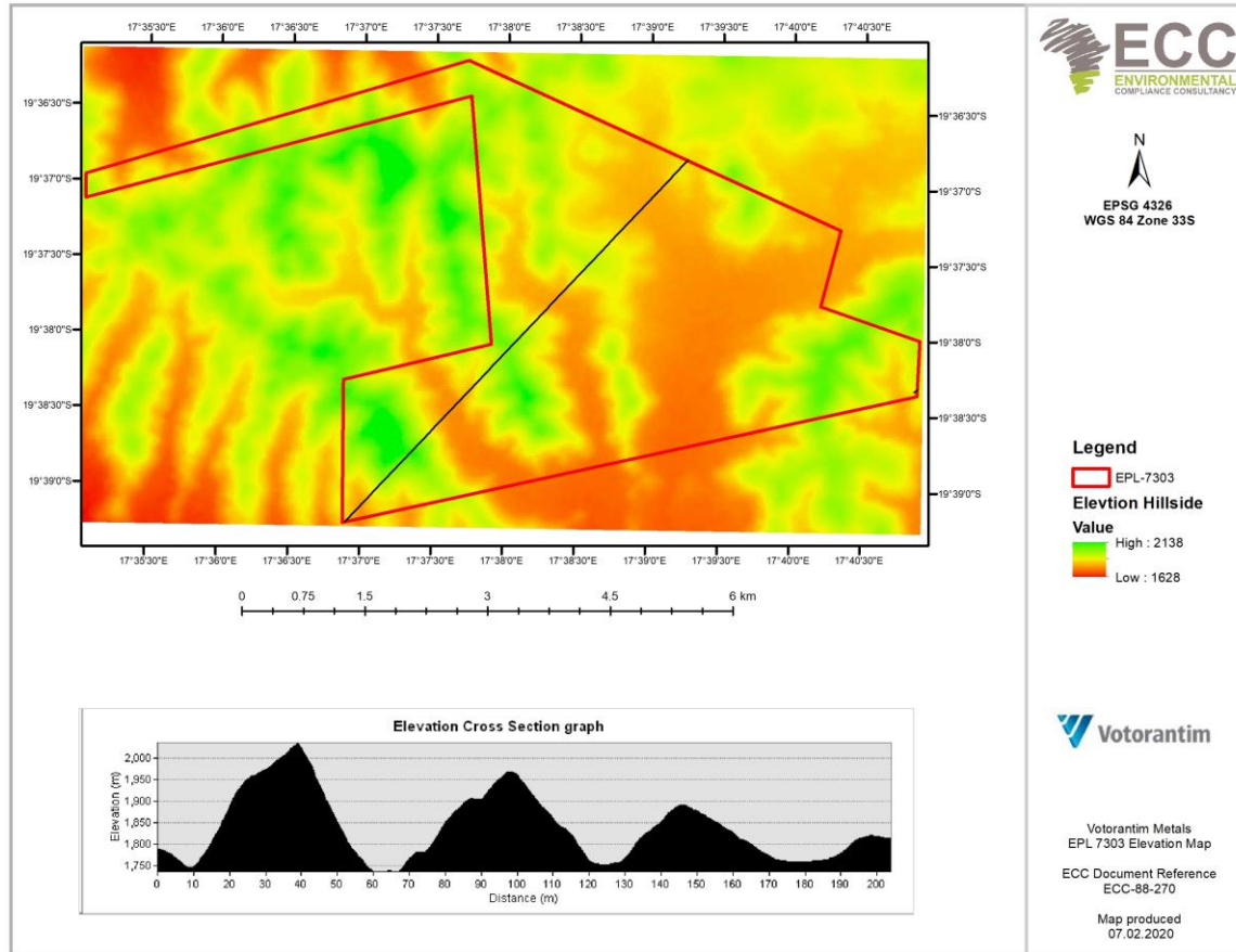
FIGURE 8 - ELEVATION PROFILE ALONG EPL 7303
