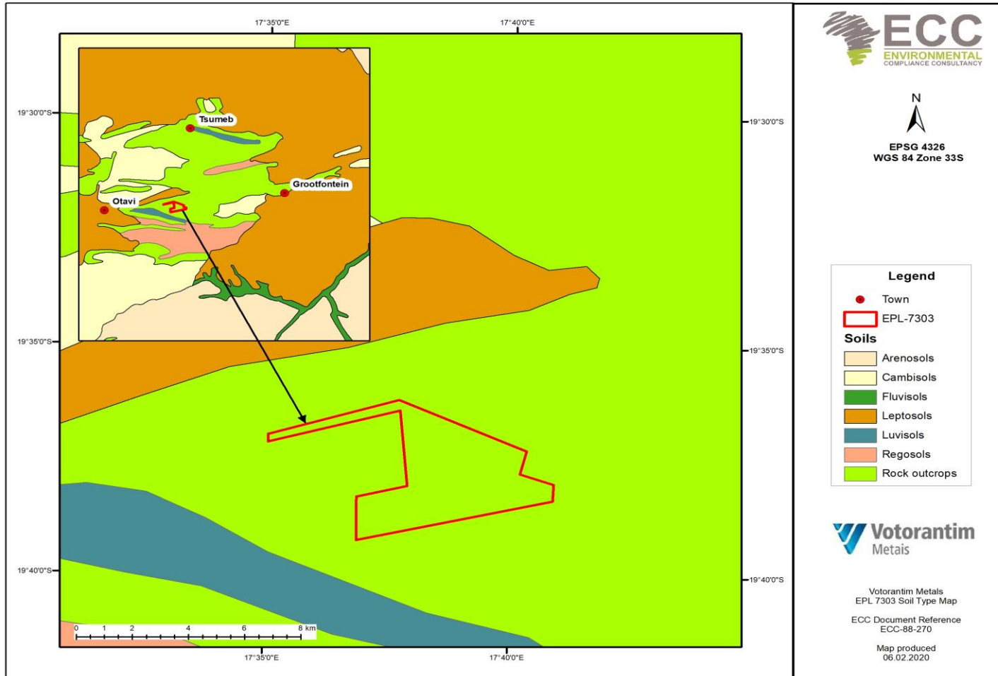
FIGURE 7 - EPL 7303 REGIONAL AND LOCAL SOIL MAP
