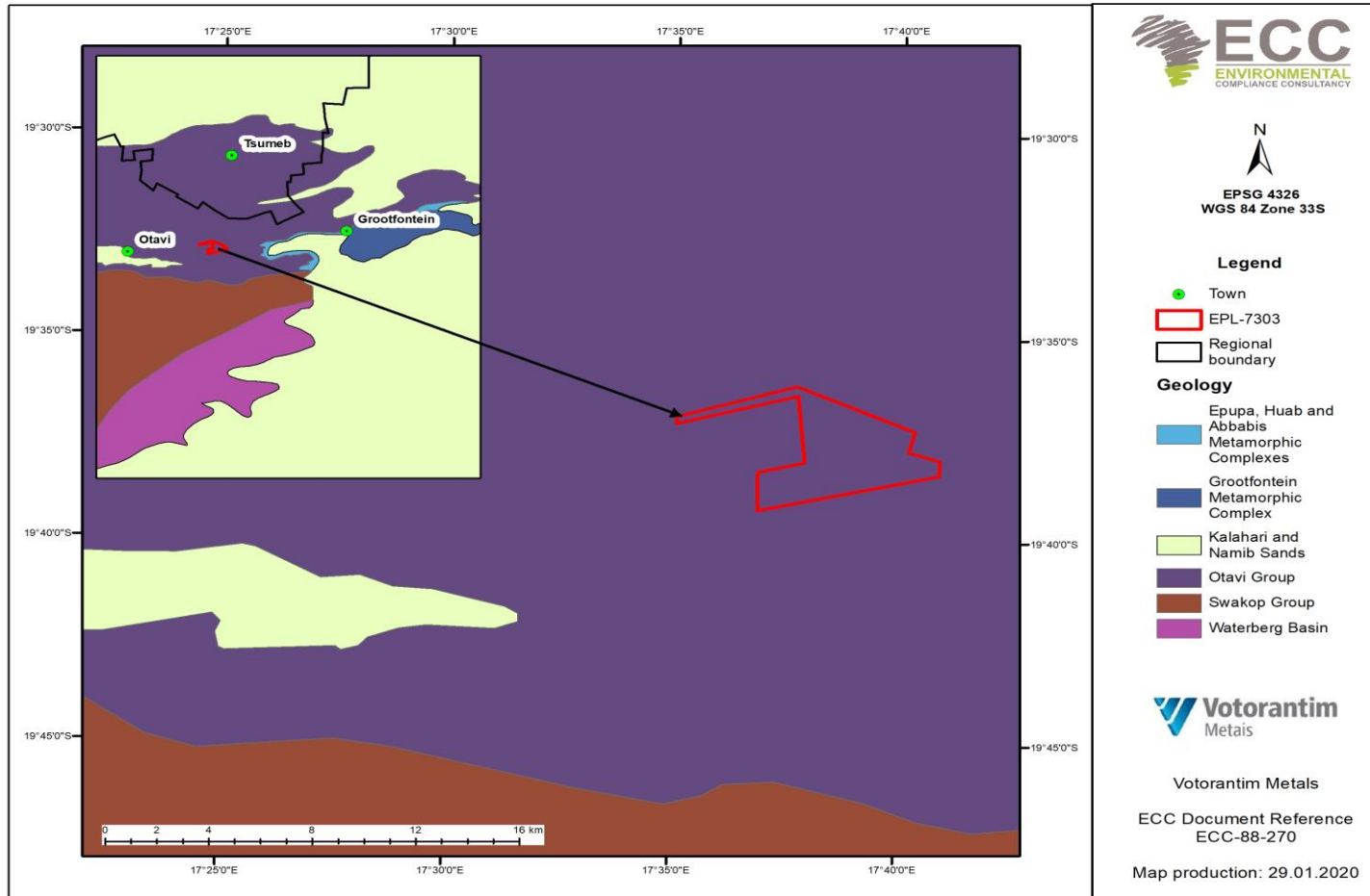
FIGURE 6 - EPL 7303 REGIONAL AND LOCAL GEOLOGY
