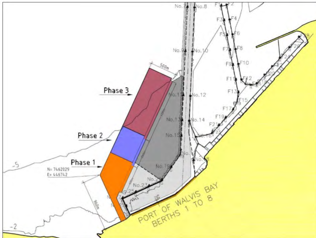
Figure 36 – Nampont Container Expansion project (Source: (Delta Marine Consultants, 2010))
