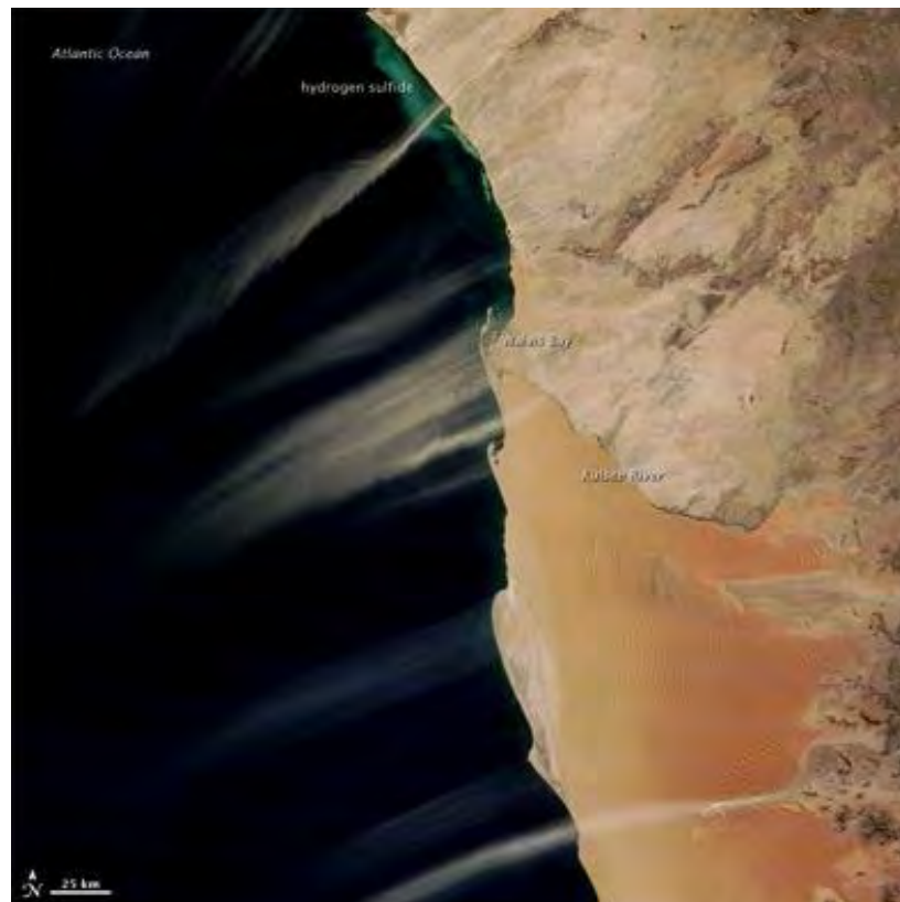
Figure 43 - Dust and Hydrogen Sulphide (green) along the Namibian coast (Source: NASA, 2010)
