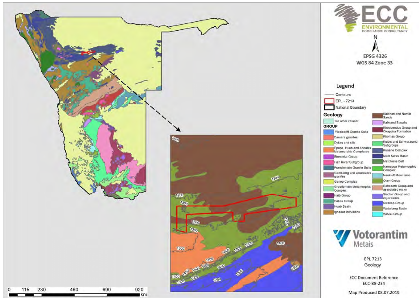
FIGURE 7 - EPL 7213 REGIONAL AND LOCAL GEOLOGY
