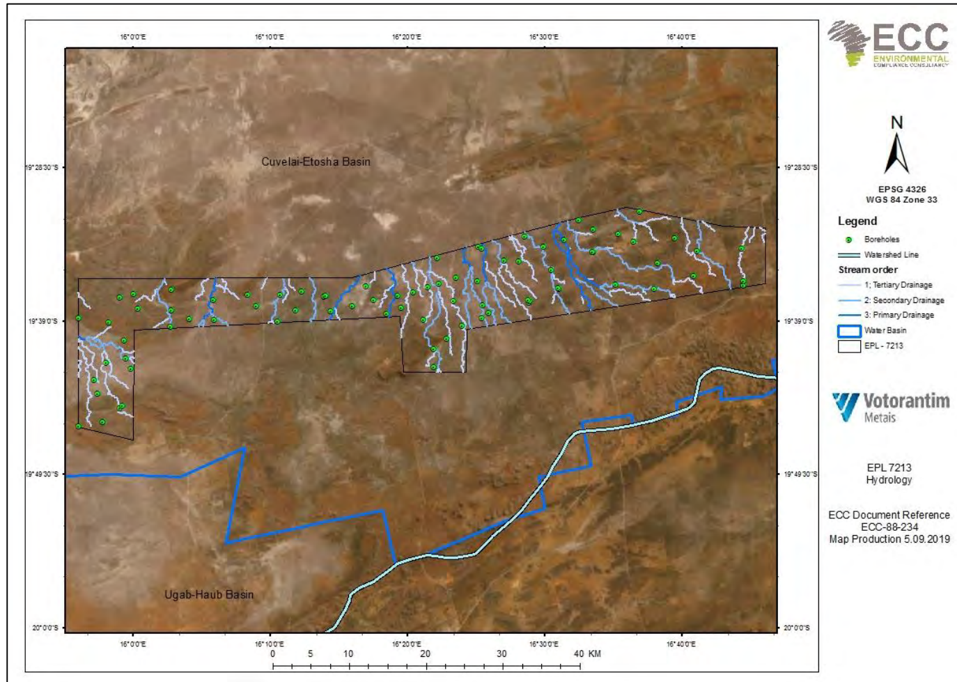
FIGURE 10 - HYDROLOGY MAP OF THE EPL 7213
