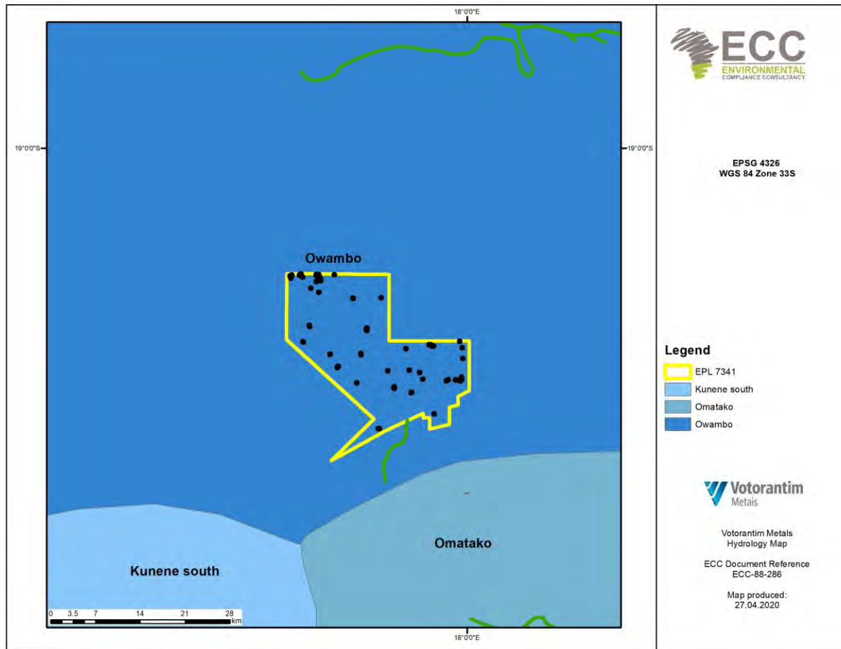
FIGURE 9 - HYDROLOGY MAP OF THE EPL 7341
