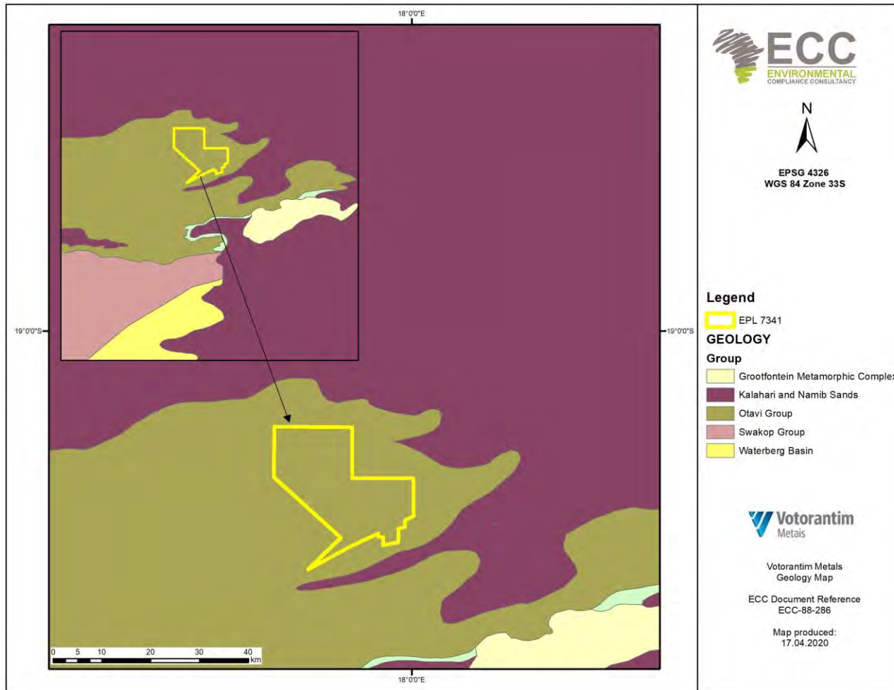
FIGURE 6 - EPL 7341 REGIONAL AND LOCAL GEOLOGY
