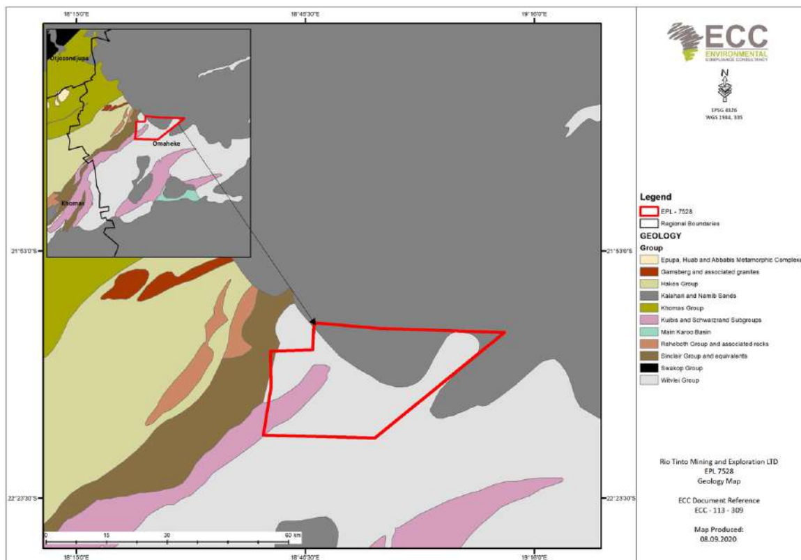
FIGURE 5 - REGIONAL GEOLOGICAL SETTING OF EPL 7528
