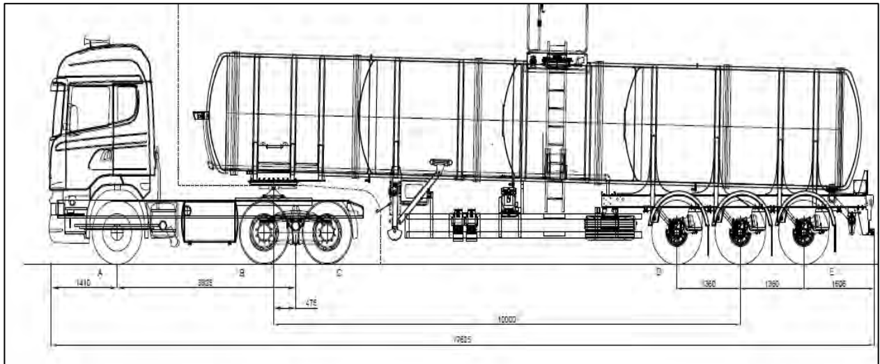
FIGURE 3 - ILLUSTRATION OF THE PROPOSED PROJECT'S TANKER TRUCKS
