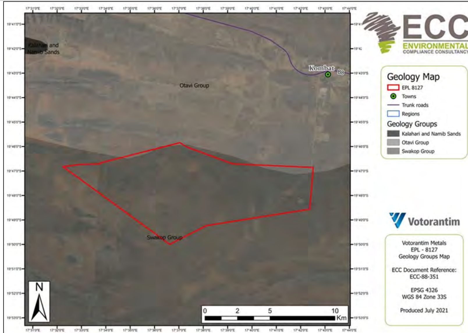
Figure 6 - EPL 8127 regional and local geology
