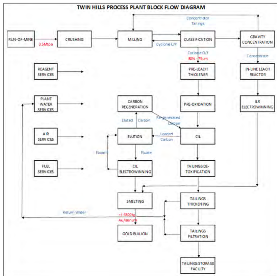
Figure 2: Twin Hills Gold Project Process Plant Flowsheet sing plant (Moeller, 2021)
