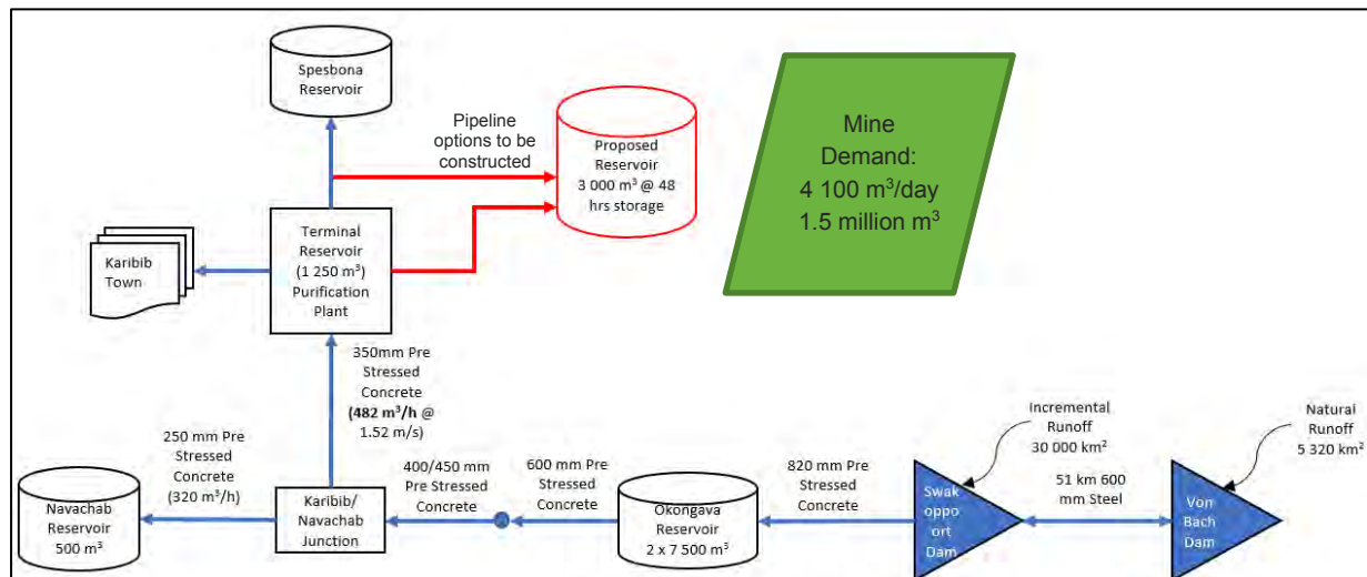
Figure 4-2 Namwater Supply Schematic
