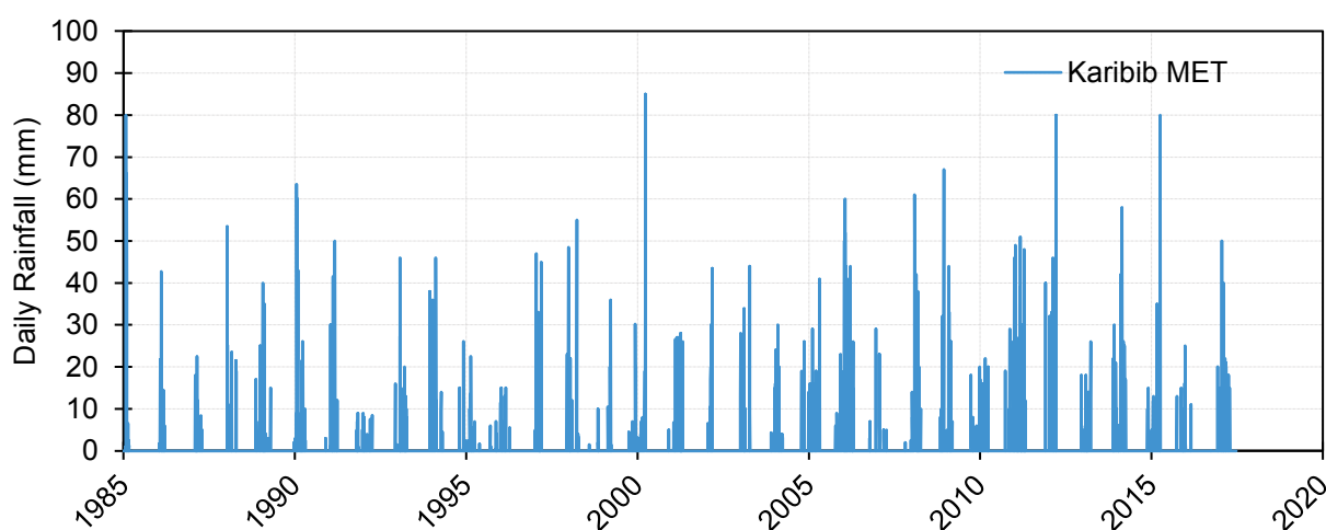
Figure 2-1 Daily Rainfall Record for the Karibib NMET Station
