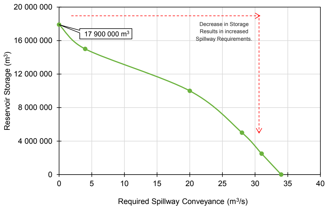
Figure 3-10 Spillway size vs storage
