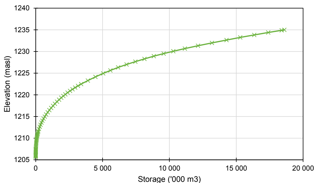
Figure 3-5 Approximate Storage-Elevation relationship Option 1
