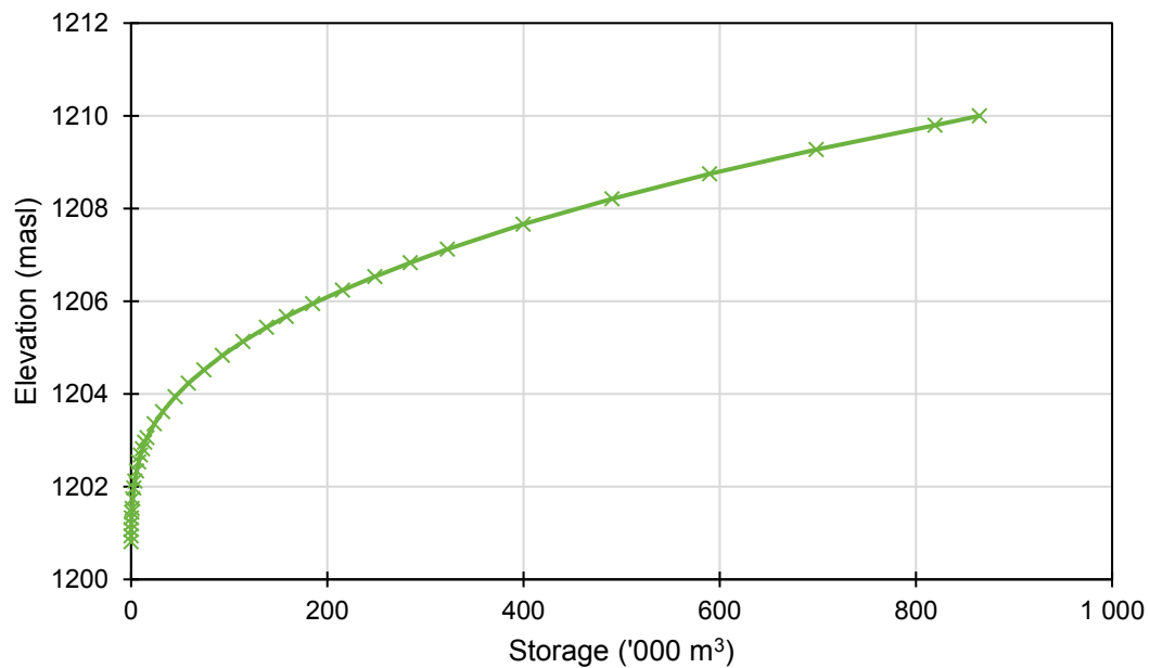
Figure 3-6 Approximate Storage-Elevation relationship Option 2
