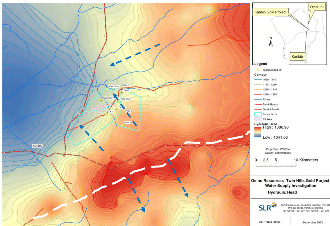
Figure 2-3: Hydraulic head and groundwater flow
