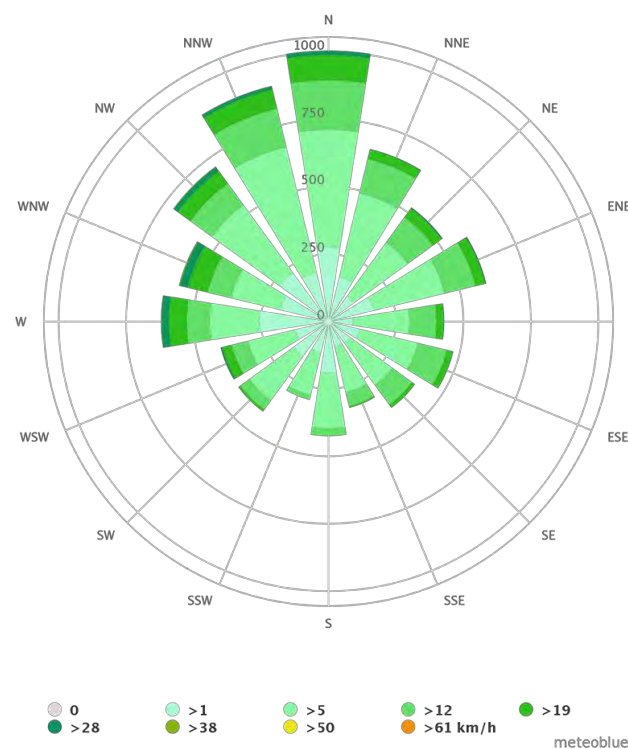
Figure 5 - Average wind speed and direction of this area
