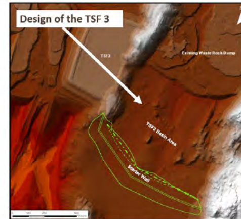
Figure 4: Plan View of Option 4 Starter Wall (Dashed Line) and Final Downstream Embankment
