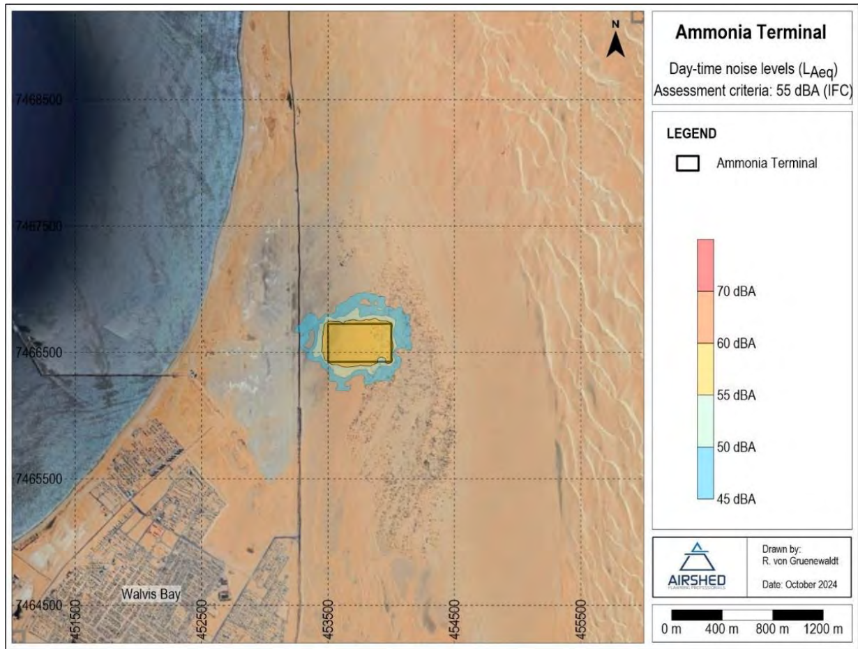
Figure 53 - Simulated day-time noise levels due to normal Project operation only
