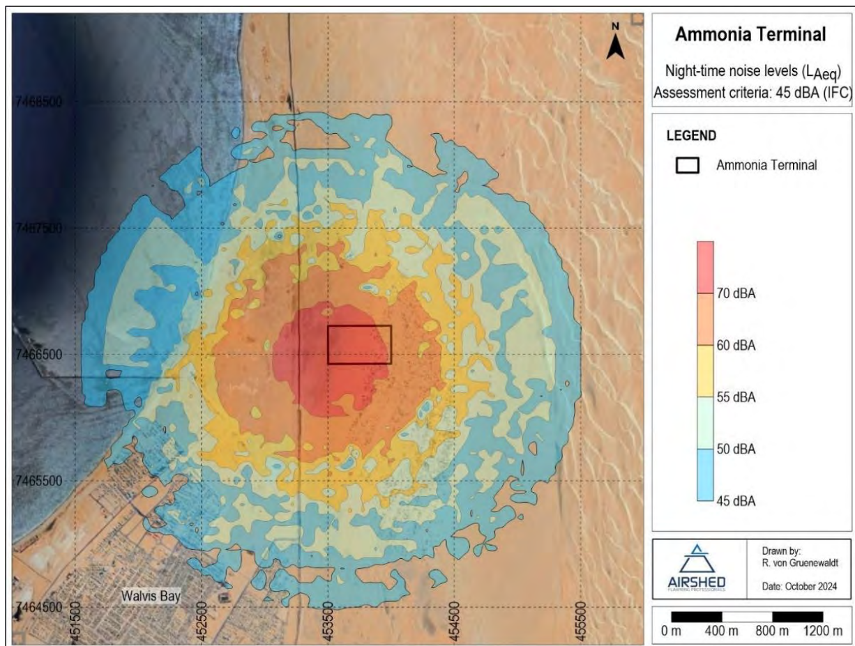
Figure 56 - Simulated night-time noise levels due to Project emergency process (assuming 1 hr tank PVs maximum release through the flare)
