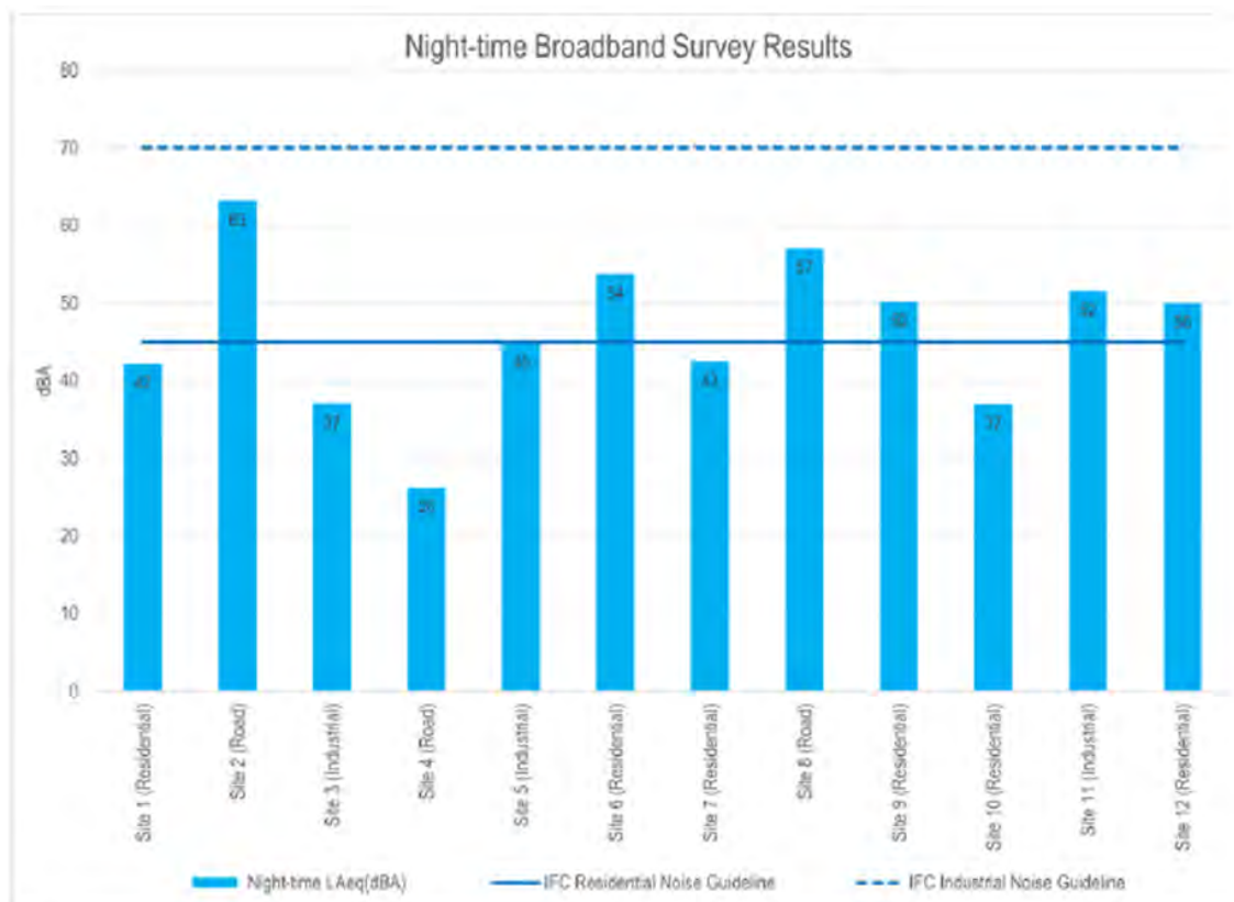
Figure 32 - Night-time broadband survey results (Airshed, 2024)
