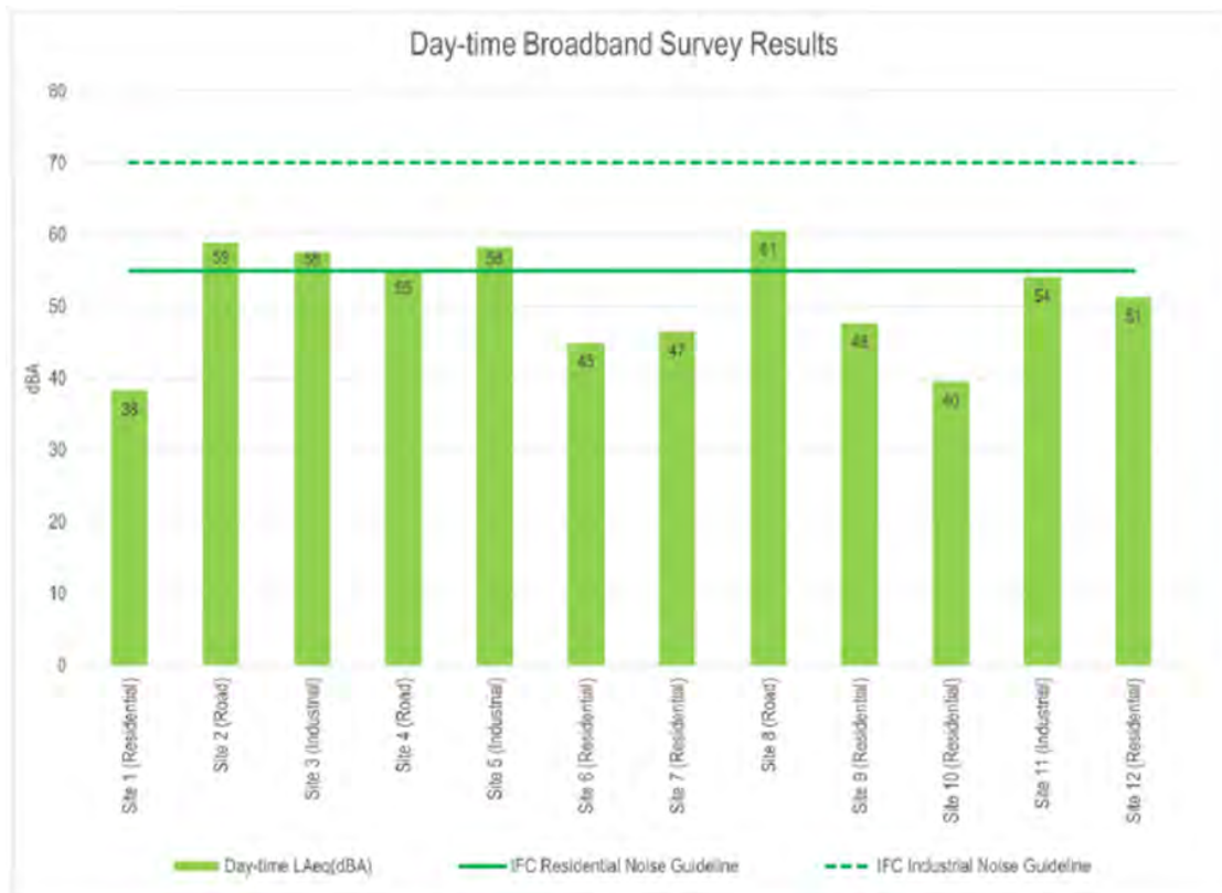
Figure 31 - Day-time broadband survey results (Airshed, 2024)
