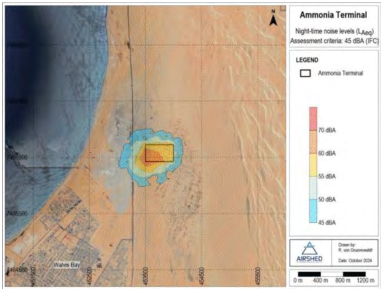
Figure 58 - Simulated night-time noise levels due to Project emergency process (assuming 1 hr scrubber emission release through the flare)
