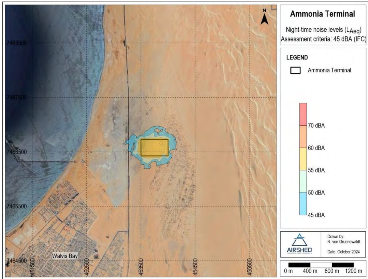
Figure 54 - Simulated night-time noise levels due to normal Project operations only
