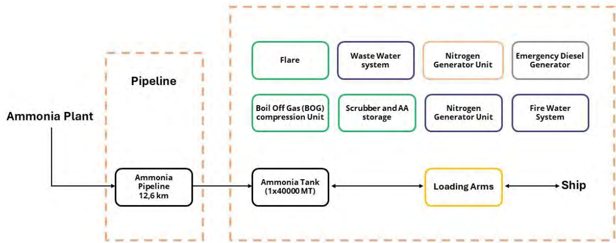
Figure 6 - Block Flow diagram of the Ammonia Terminal
