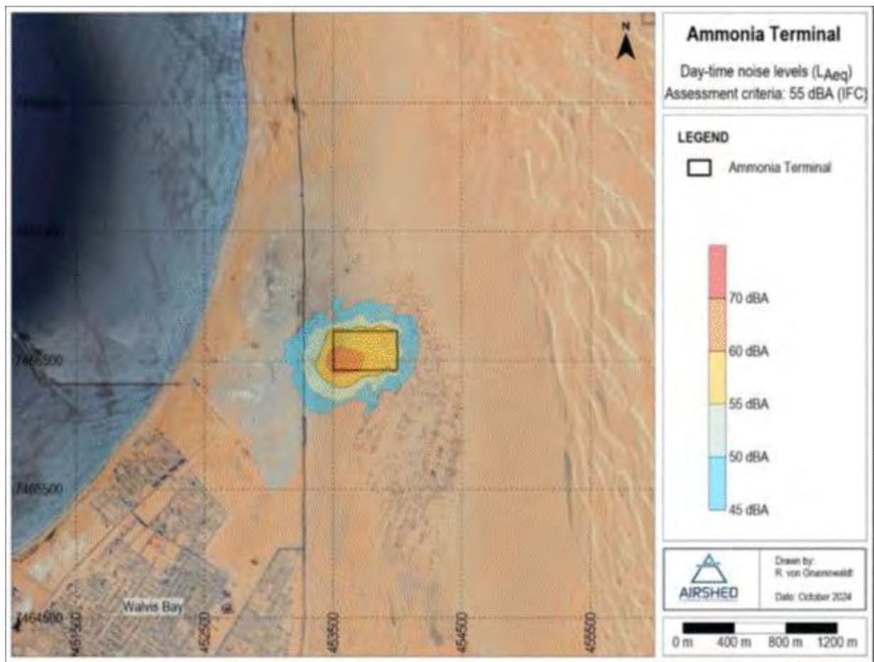
Figure 57 - Simulated day-time noise levels due to Project emergency process (assuming 1 hr scrubber emission release through the flare)
