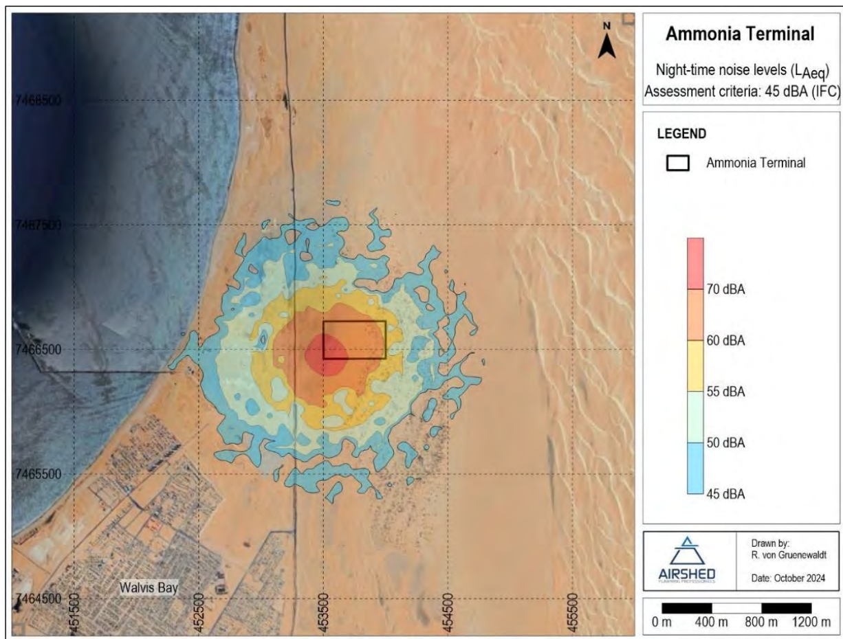
Figure 60 - Simulated night-time noise levels due to Project during commissioning operations only
