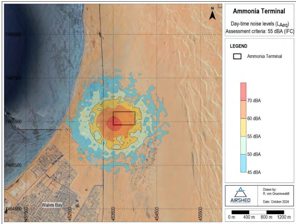
Figure 59 - Simulated day-time noise levels due to Project during commissioning operations only
