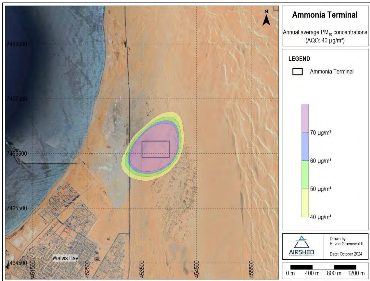
Figure 40 - Simulate annual average PM 10 ground level concentrations due to Project construction activities
