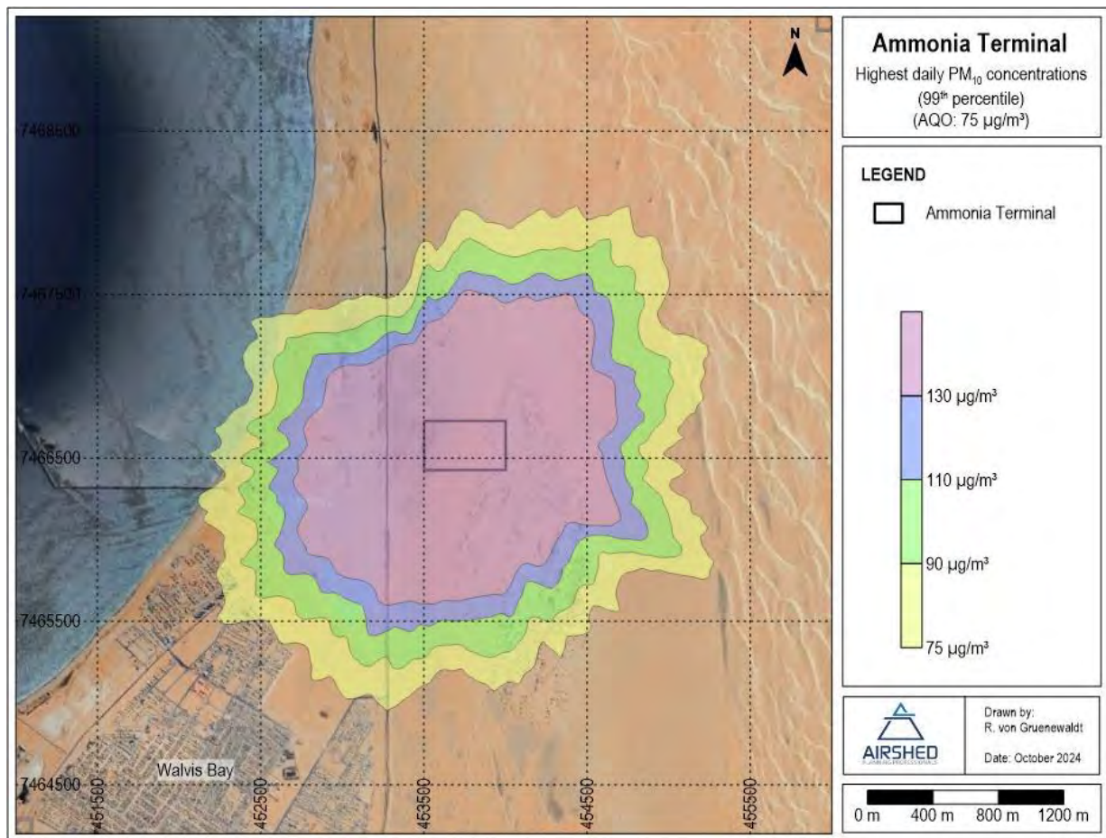
Figure 39 - Simulate daily (99th percentile) PM 10 ground level concentrations due to Project construction activities
