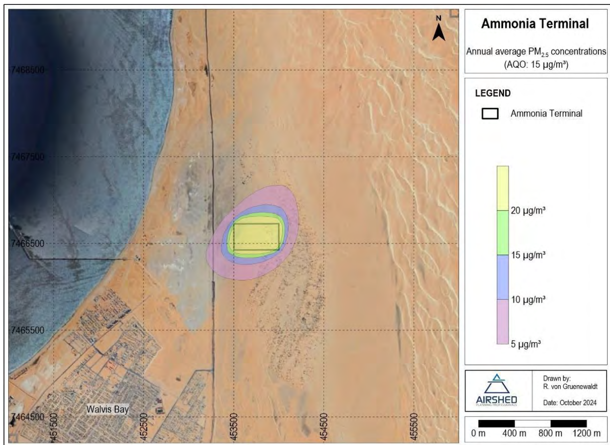
Figure 38 - Simulate annual average PM 2.5 ground level concentrations due to Project activities
