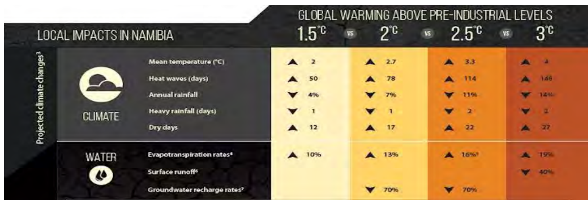
Figure 68 - What global warming of 1.5 °C and higher means for Namibia (New, 2018)
