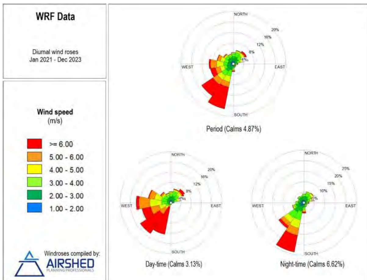
Figure 12 - Period, day - and night-time wind roses based on modelled WRF data (Airshed, 2024)
