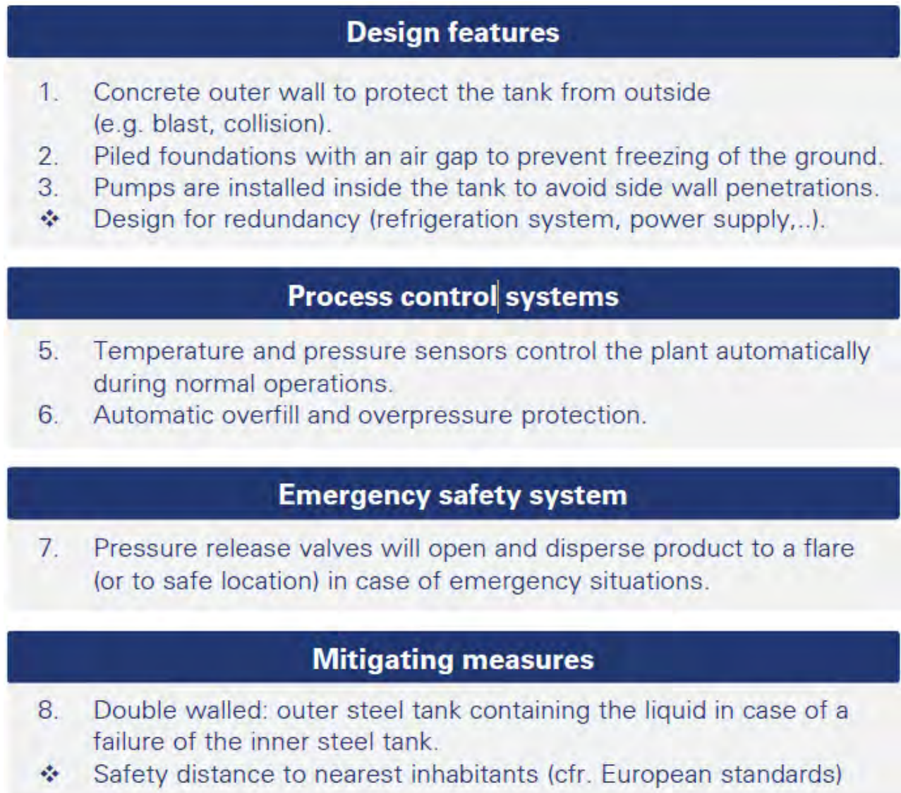
Figure 5 - Ammonia terminal design (a); Descriptions to the labelled components of the Ammonia Terminal structure (b), (Source: Cleanergy Solutions)
