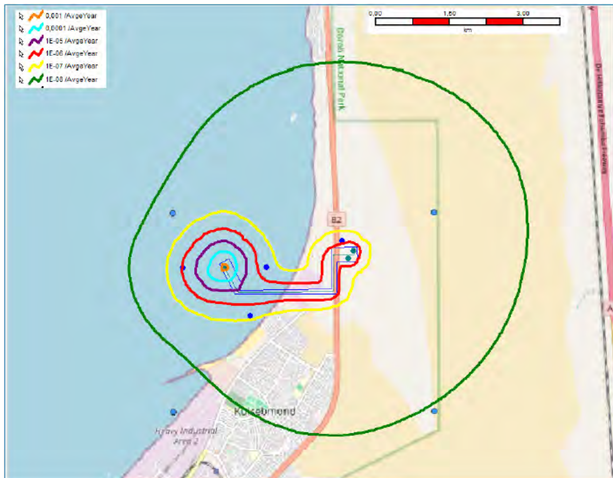
Figure 25 - Risk contours of Ammonia Terminal and operations during the first 5 years (a); Risk contours of Ammonia Terminal with export after the initial 5 years (b)
