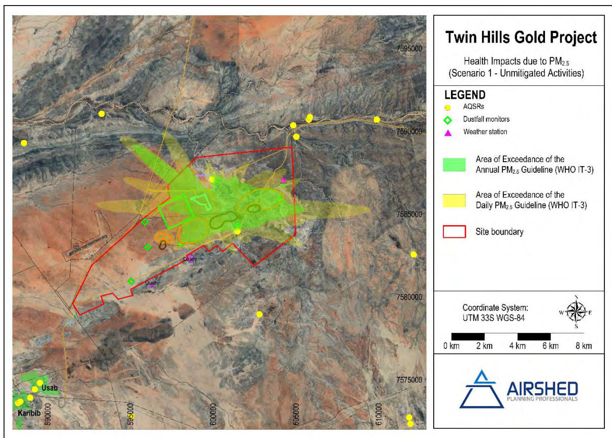
Figure 13: Area of non-compliance of daily and annual PM 2.5 AQO for unmitigated Year 6 operations
