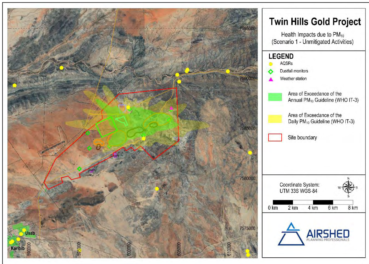
Figure 11: Area of non-compliance of daily and annual PM 10 AQO for unmitigated Year 6 operations
