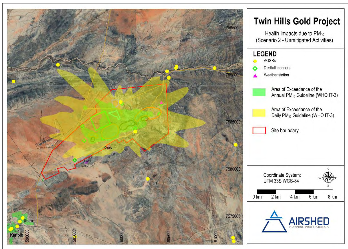
Figure 17: Area of non-compliance of daily and annual PM 10 AQO for unmitigated Year 8 operations
