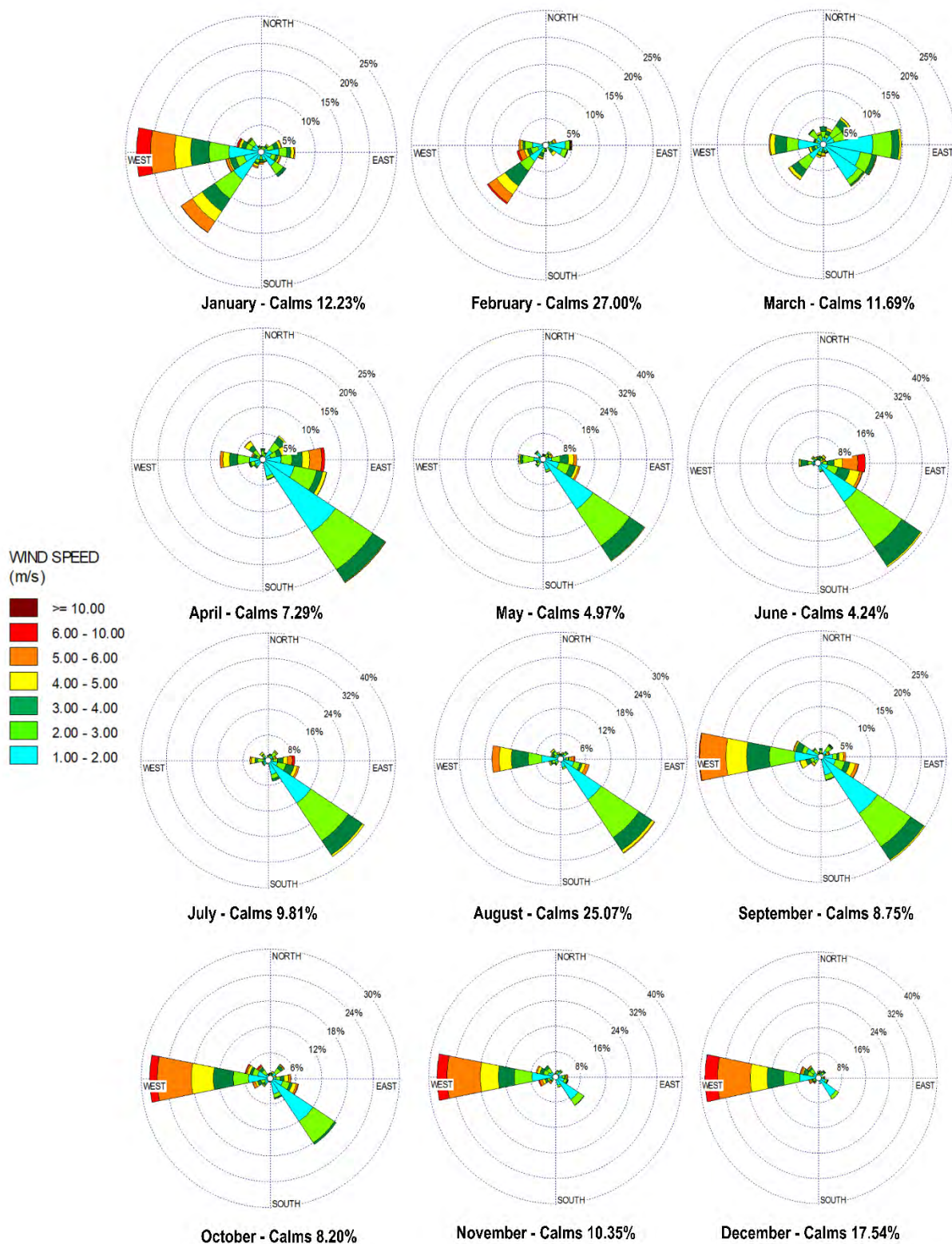
Figure 5: Monthly wind roses based on Twin Hills on-site weather data (1 January 2021 to 31 December 2022)
