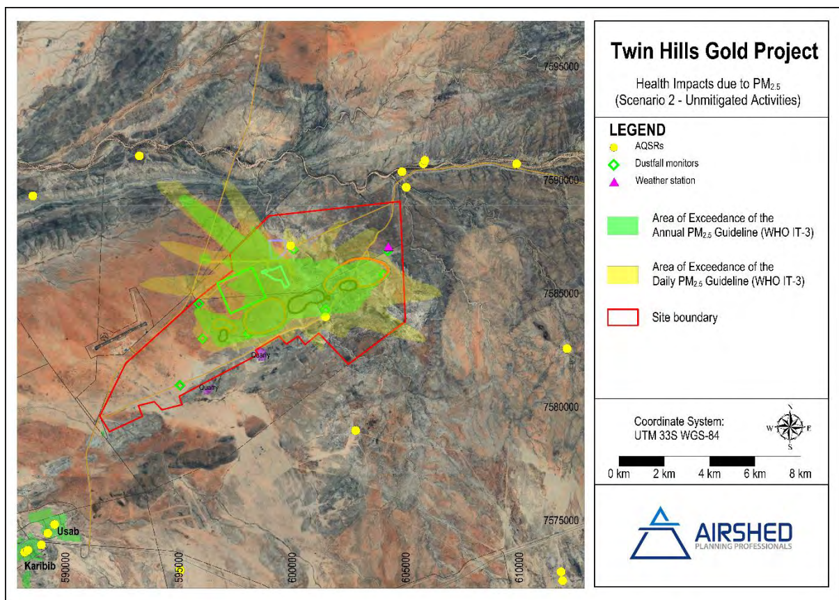
Figure 19: Area of non-compliance of daily and annual PM 2.5 AQO for unmitigated Year 8 operations
