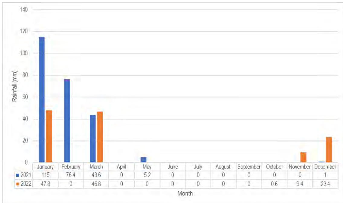
Figure 8: Average rainfall based on Twin Hills meteorological data (1 January 2021 to 31 December 2022)
