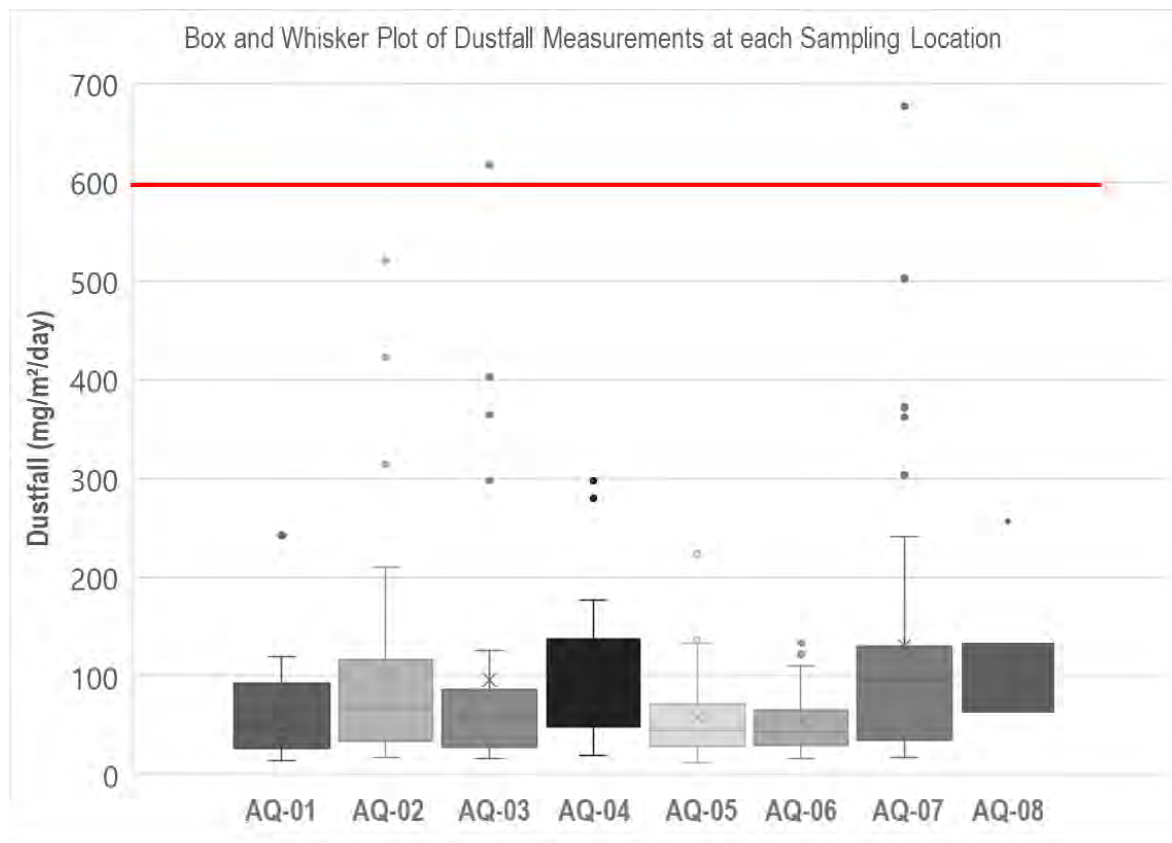
Figure 10: Box and whisker plot of the dustfall measurements at each measurement location
