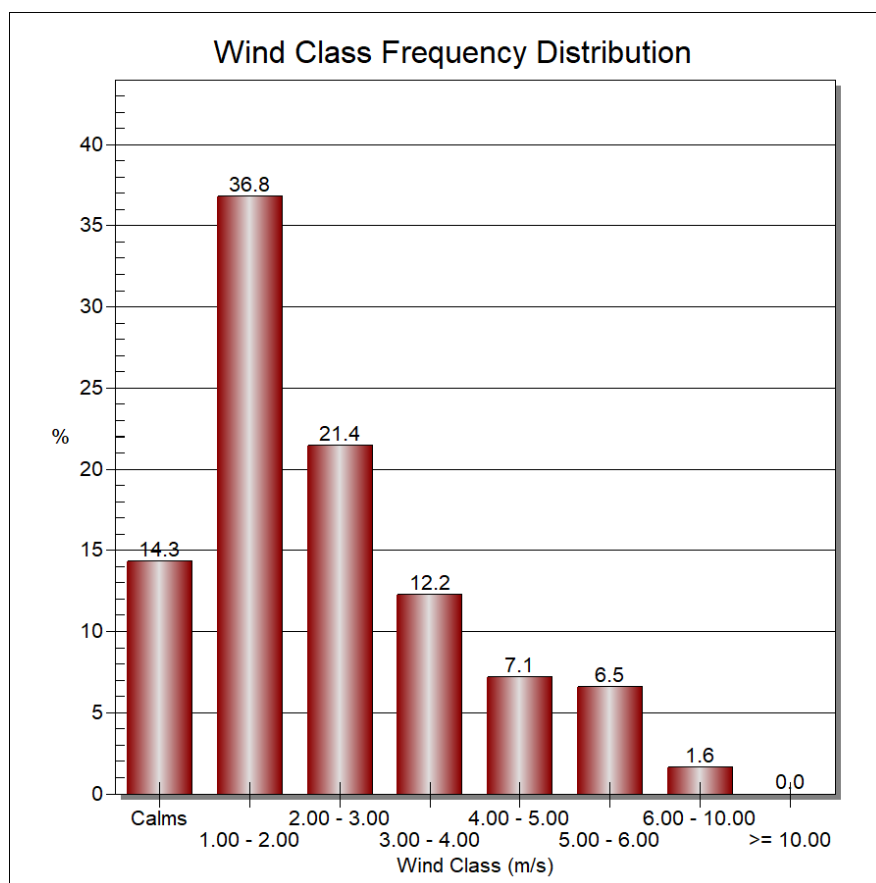
Figure 6: Wind speed categories based Twin Hills meteorological data (1 January 2021 to 31 December 2022)
