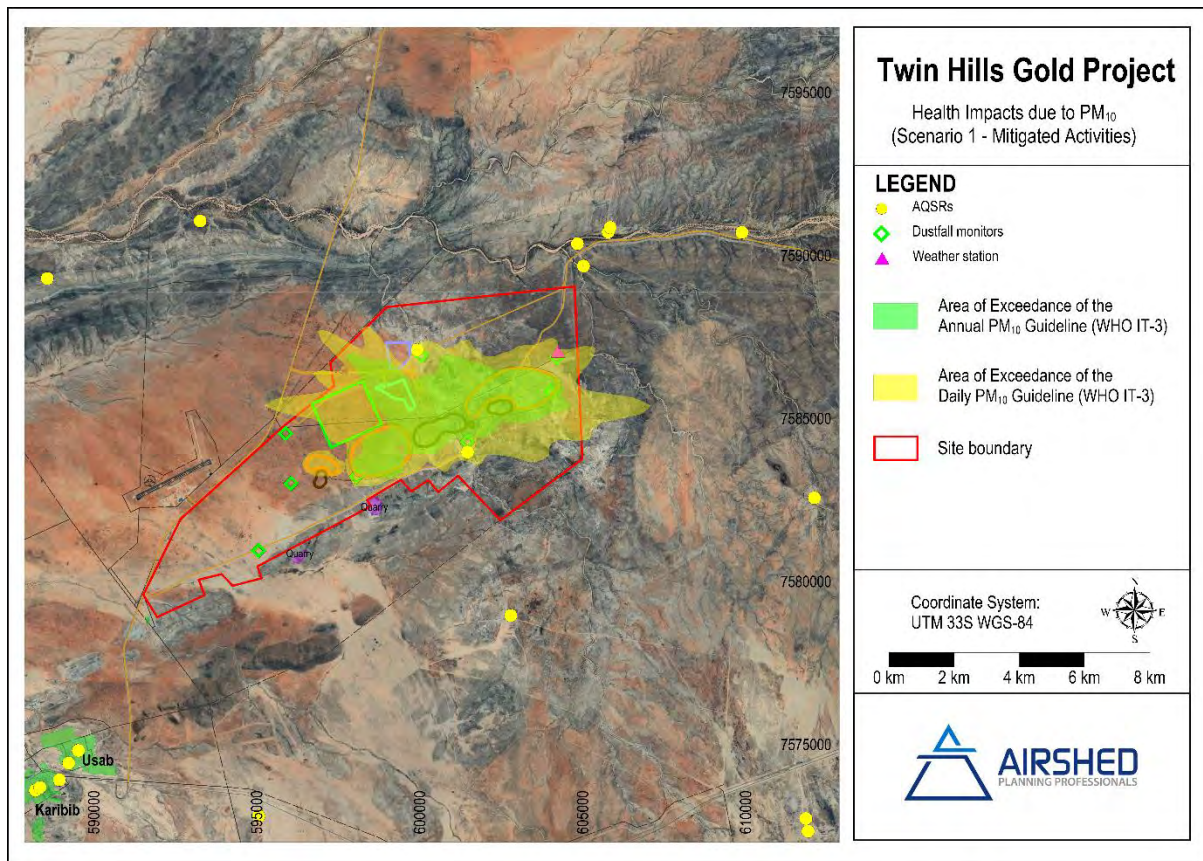
Figure 12: Area of non-compliance of daily and annual PM 10 AQO for mitigated Year 6 operations
