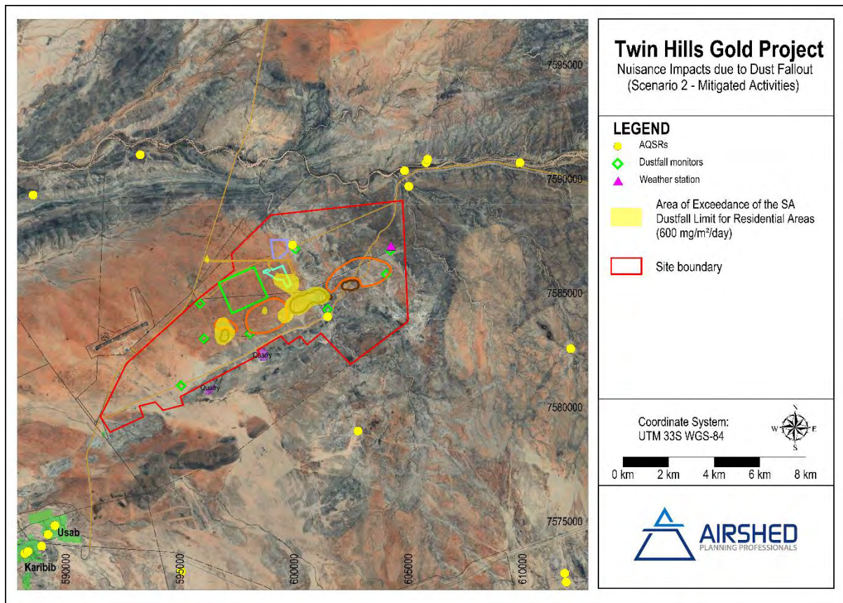
Figure 22: Area of non-compliance of dustfall limit values for mitigated Year 8 operations
