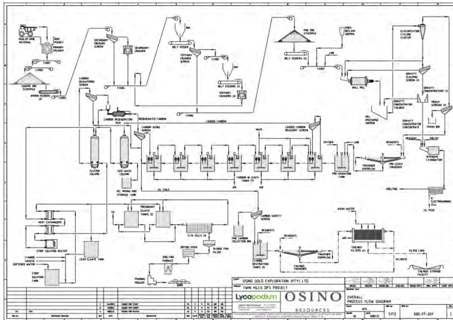
Figure 2: Twin Hills Gold Project Process Plant Flowsheet (Armstrong 2023)
