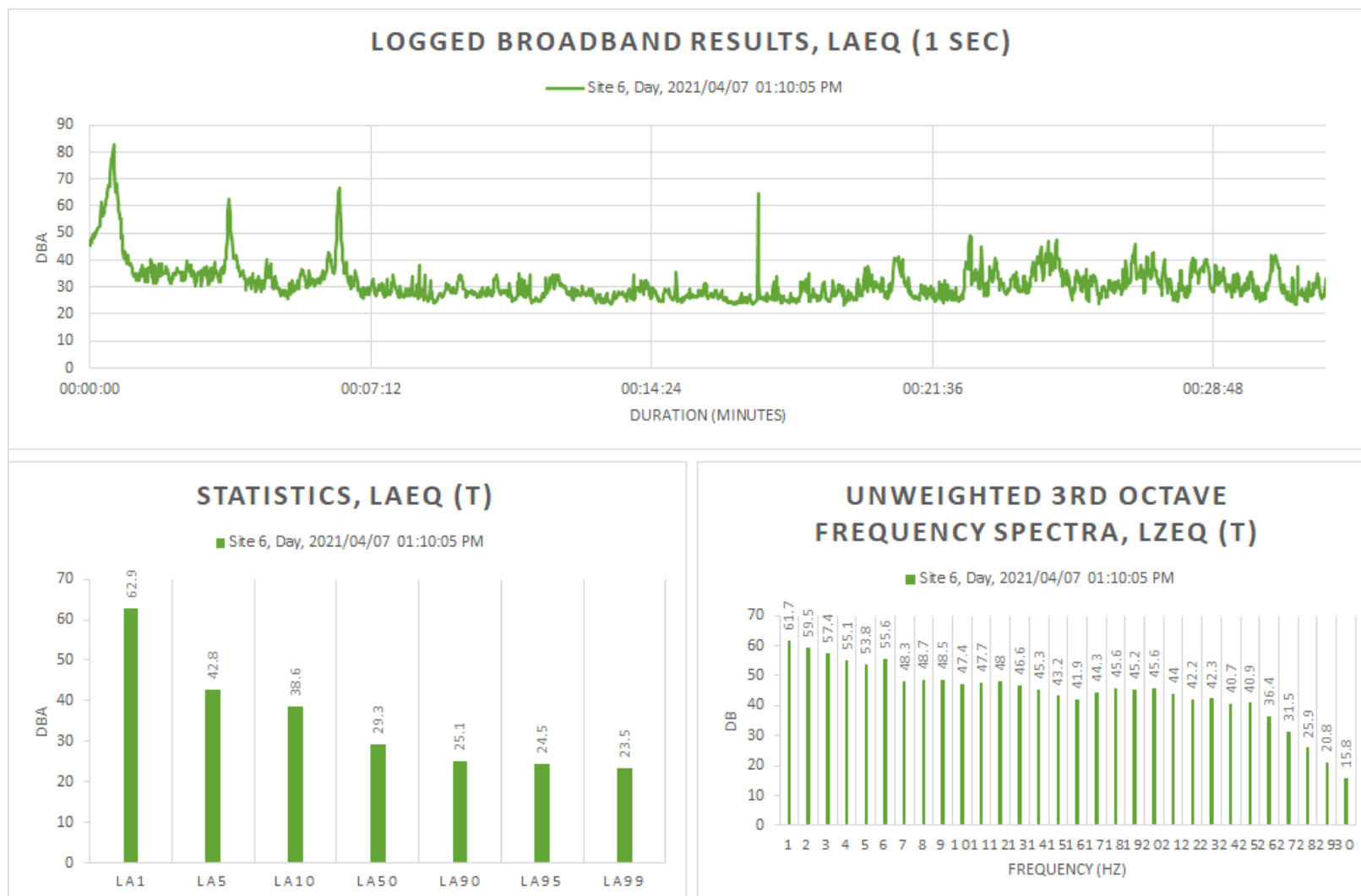
Figure 16: Detailed day-time survey results for Site 6
