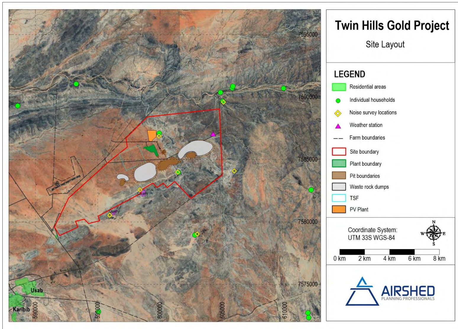
Figure 3: Twin Hills Gold Project site layout and sensitive receptors within the study area
