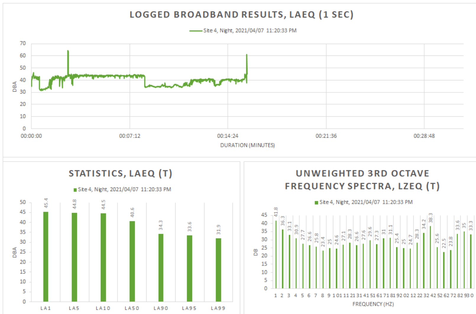
Figure 21: Detailed night -time survey results for Site 4
