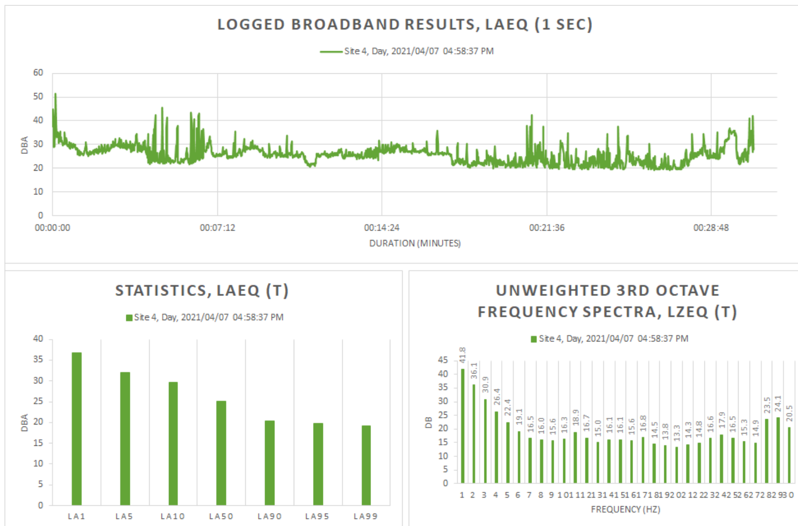
Figure 14: Detailed day-time survey results for Site 4
