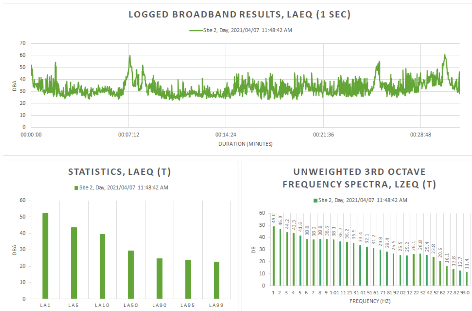
Figure 12: Detailed day-time survey results for Site 2
