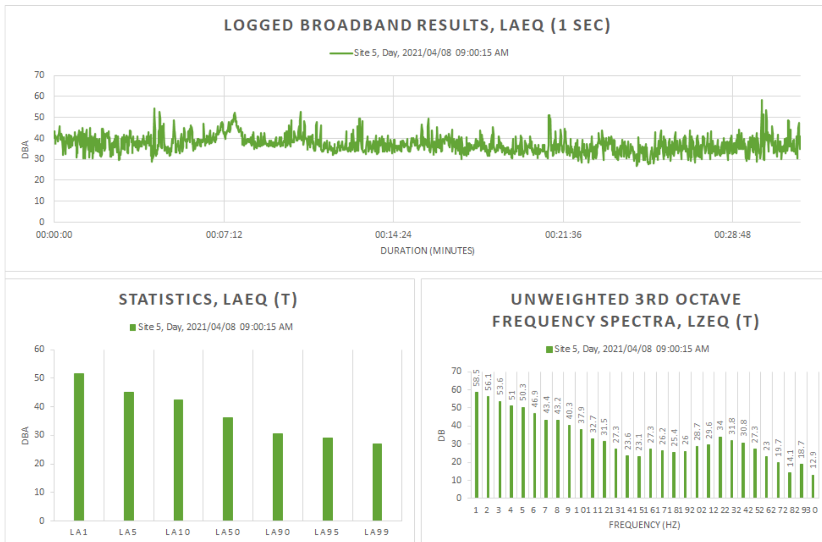
Figure 15: Detailed day-time survey results for Site 5
