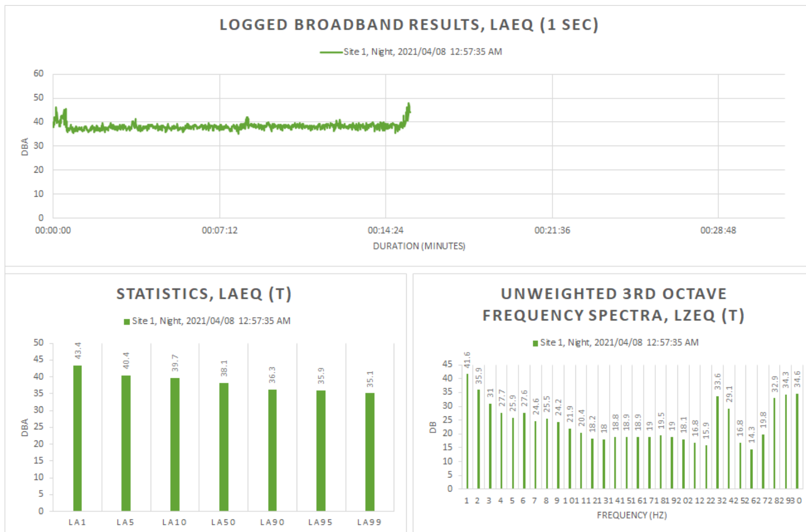
Figure 18: Detailed night-time survey results for Site 1
