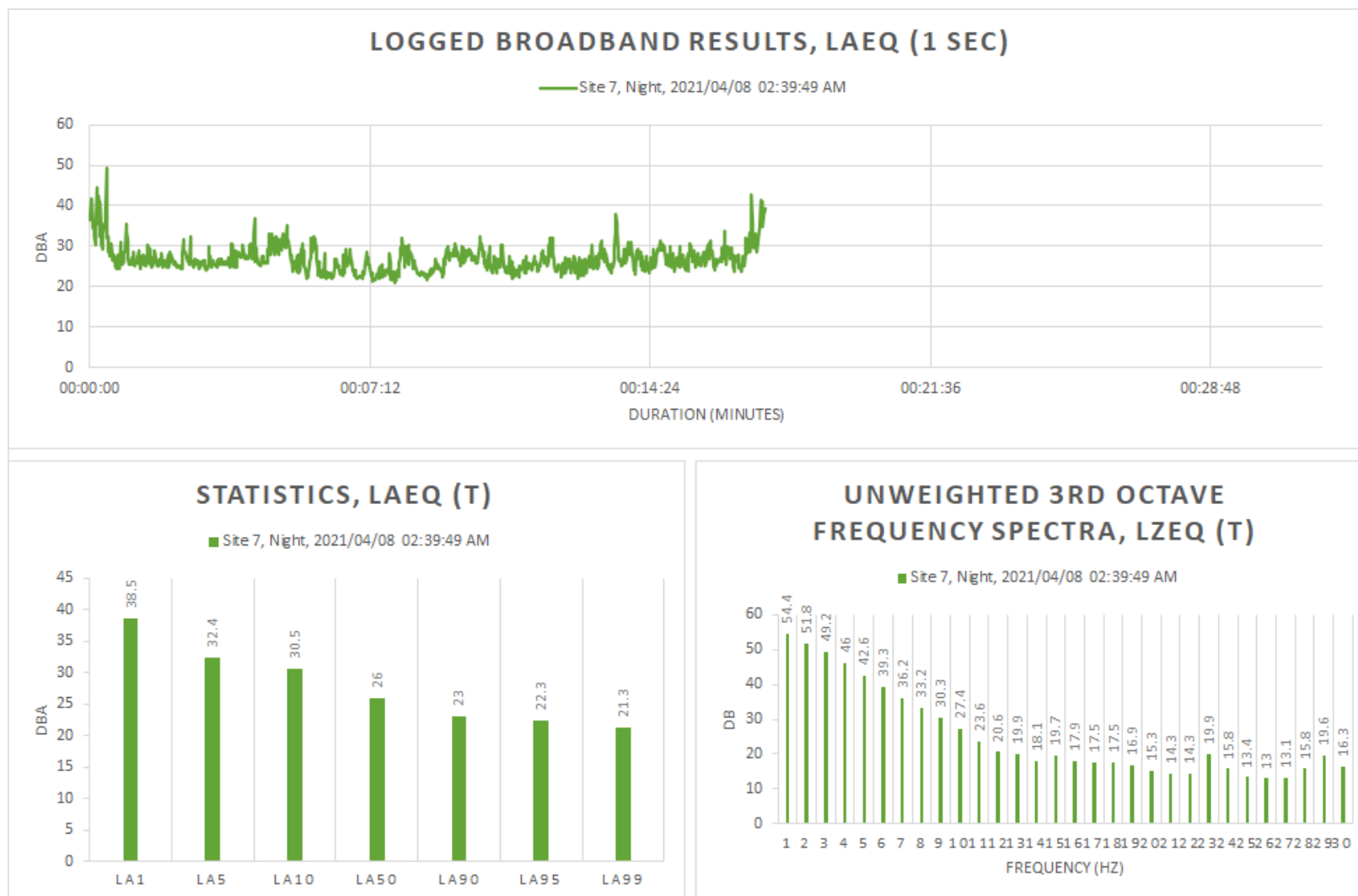
Figure 24: Detailed night -time survey results for Site 7
