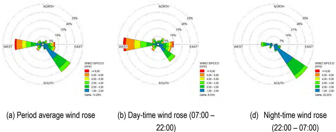
Figure 4: Wind rose for on-site station for the period 2021 to 2022
