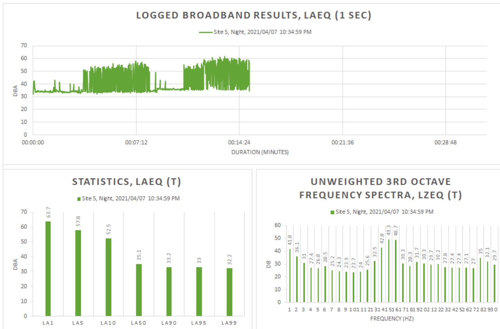
Figure 22: Detailed night -time survey results for Site 5
