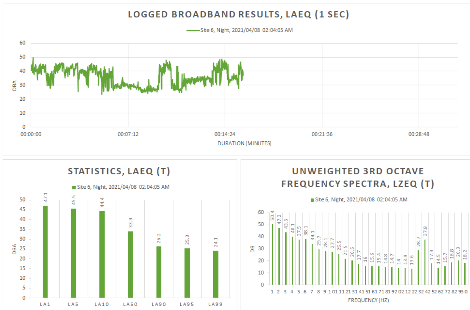
Figure 23: Detailed night -time survey results for Site 6
