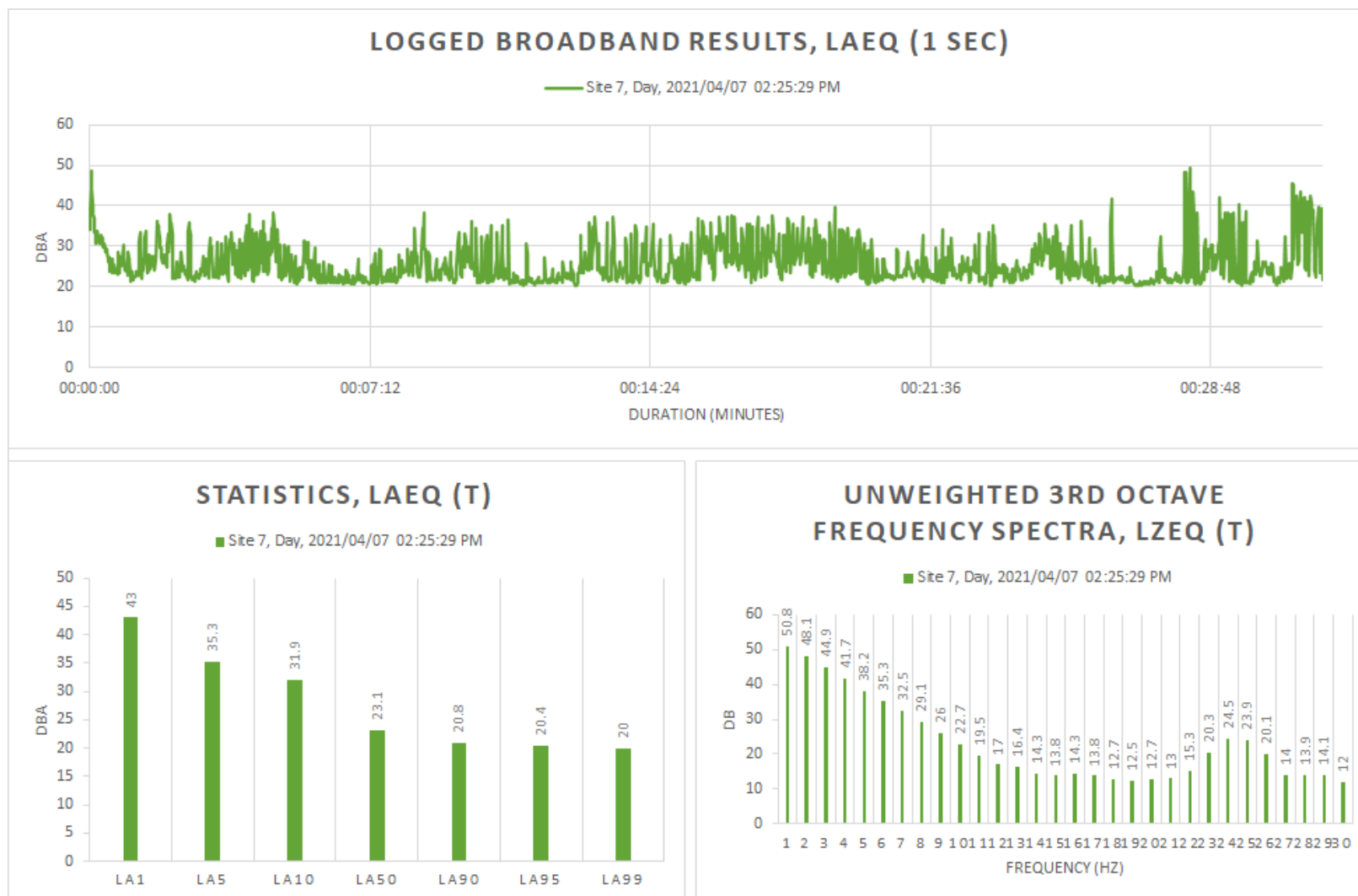
Figure 17: Detailed day-time survey results for Site 7
