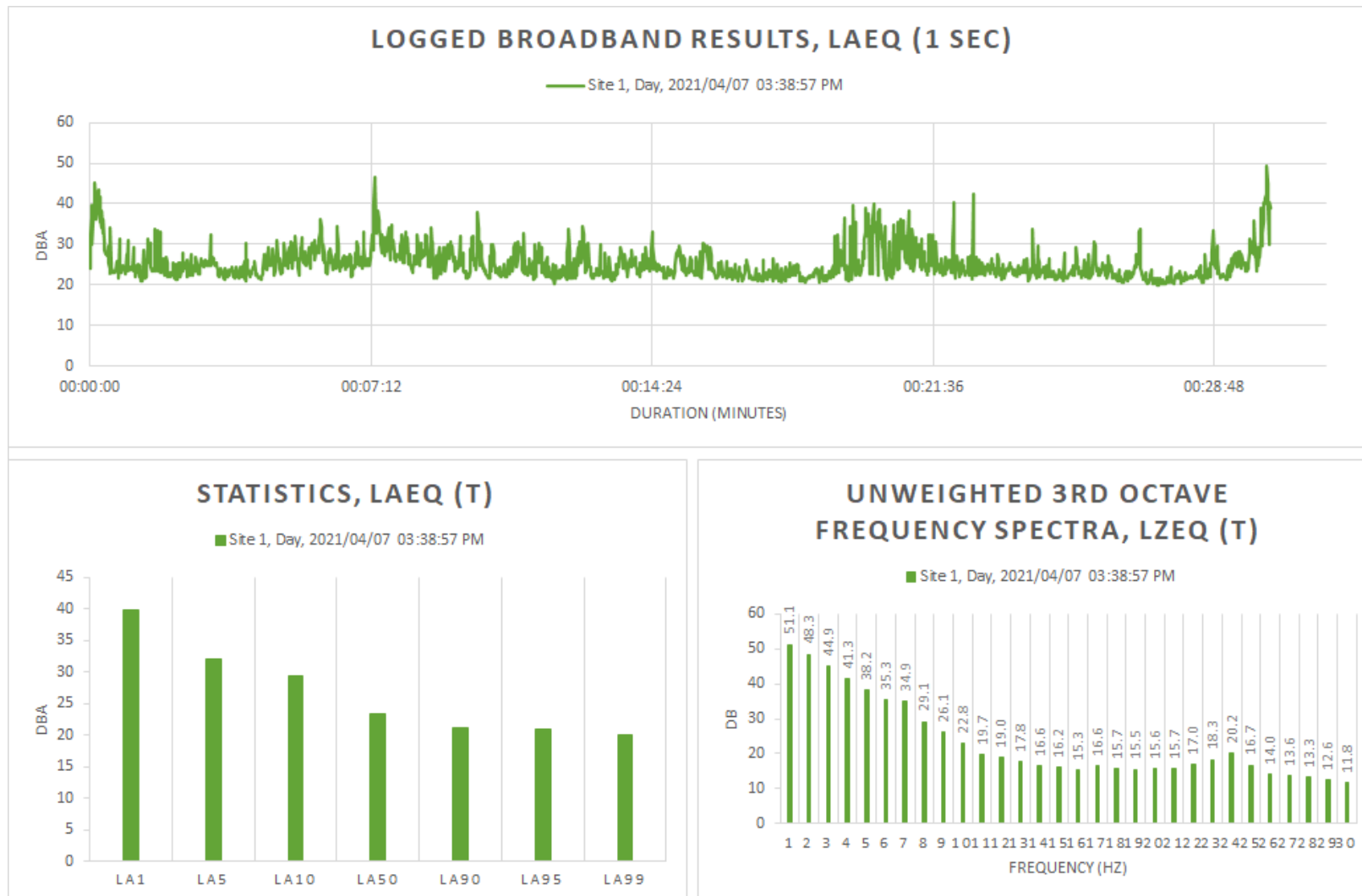
Figure 11: Detailed day-time survey results for Site 1
