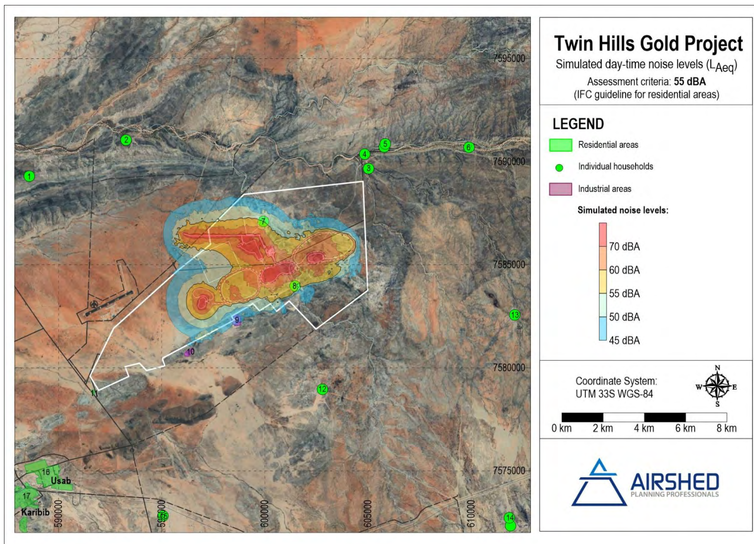
Figure 9: Simulated day-time noise levels for the project operational activities (operational Year 7)
