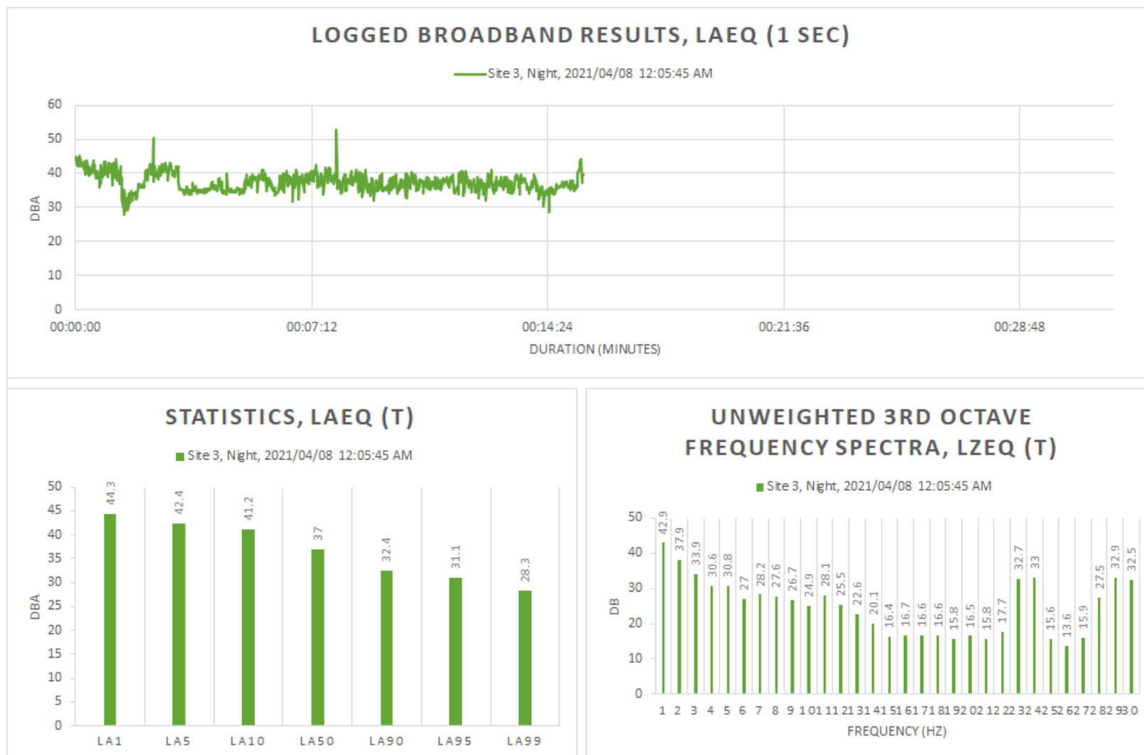
Figure 20: Detailed night -time survey results for Site 3
