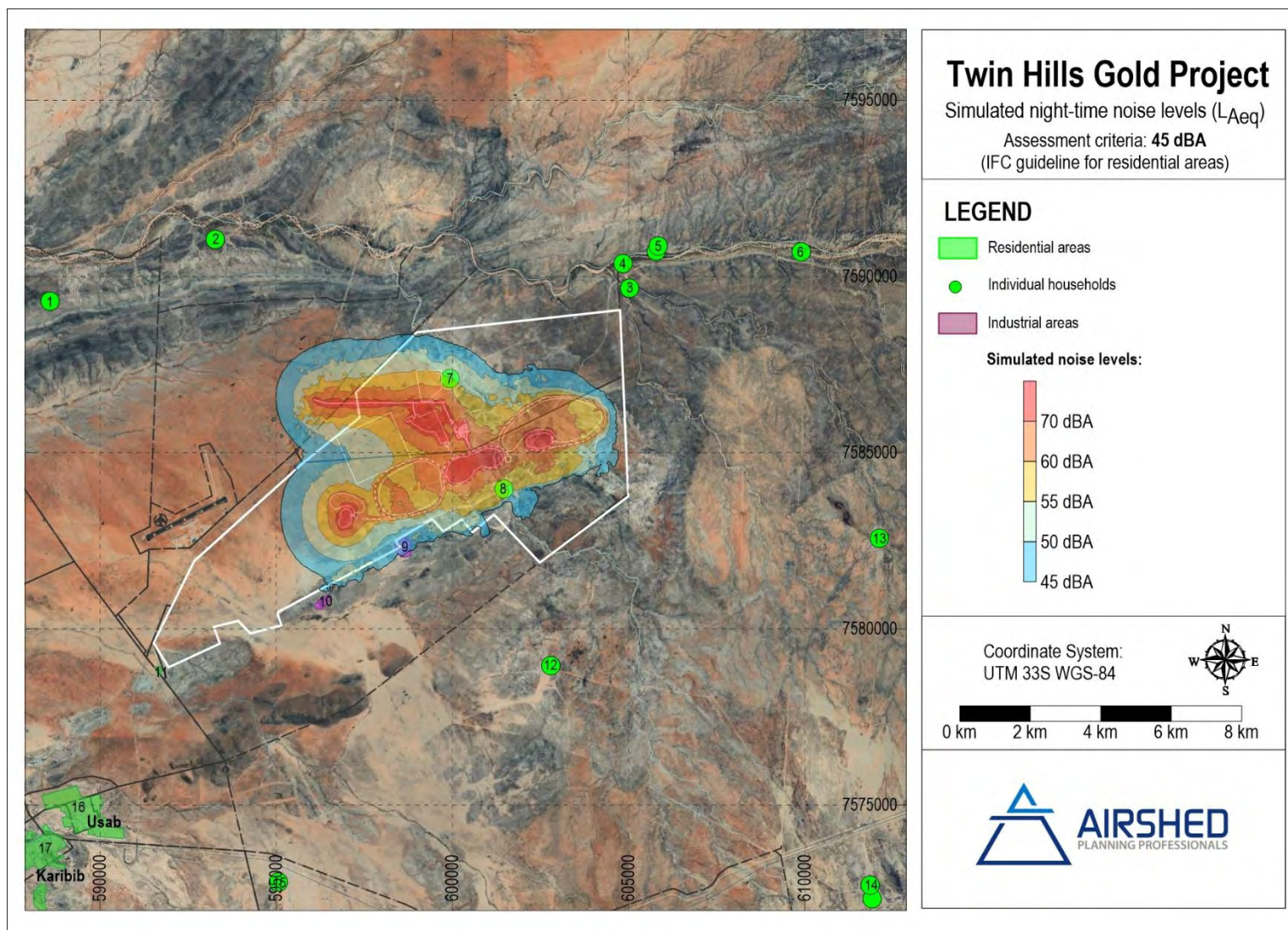
Figure 10: Simulated night-time noise levels for the project operational activities (operational Year 7)
