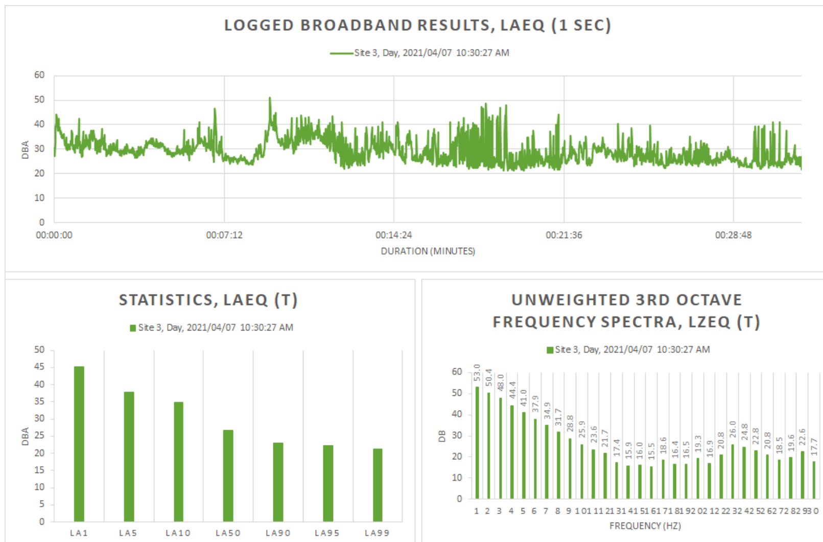
Figure 13: Detailed day-time survey results for Site 3
