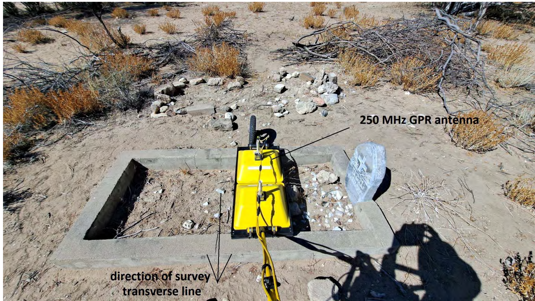
Figure 5: GPR Line 2 crossing grave 2. Note the loss of contact (coupling) with the ground
